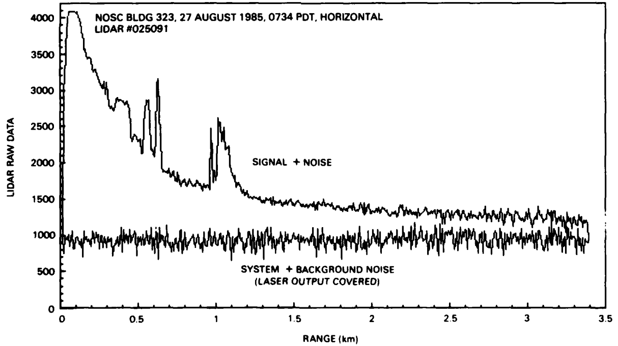
Figure 1. Comparisons of raw data plots for normal operation of the lidars and plots made when the laser outputs were covered. Visibility was about 10 km.
