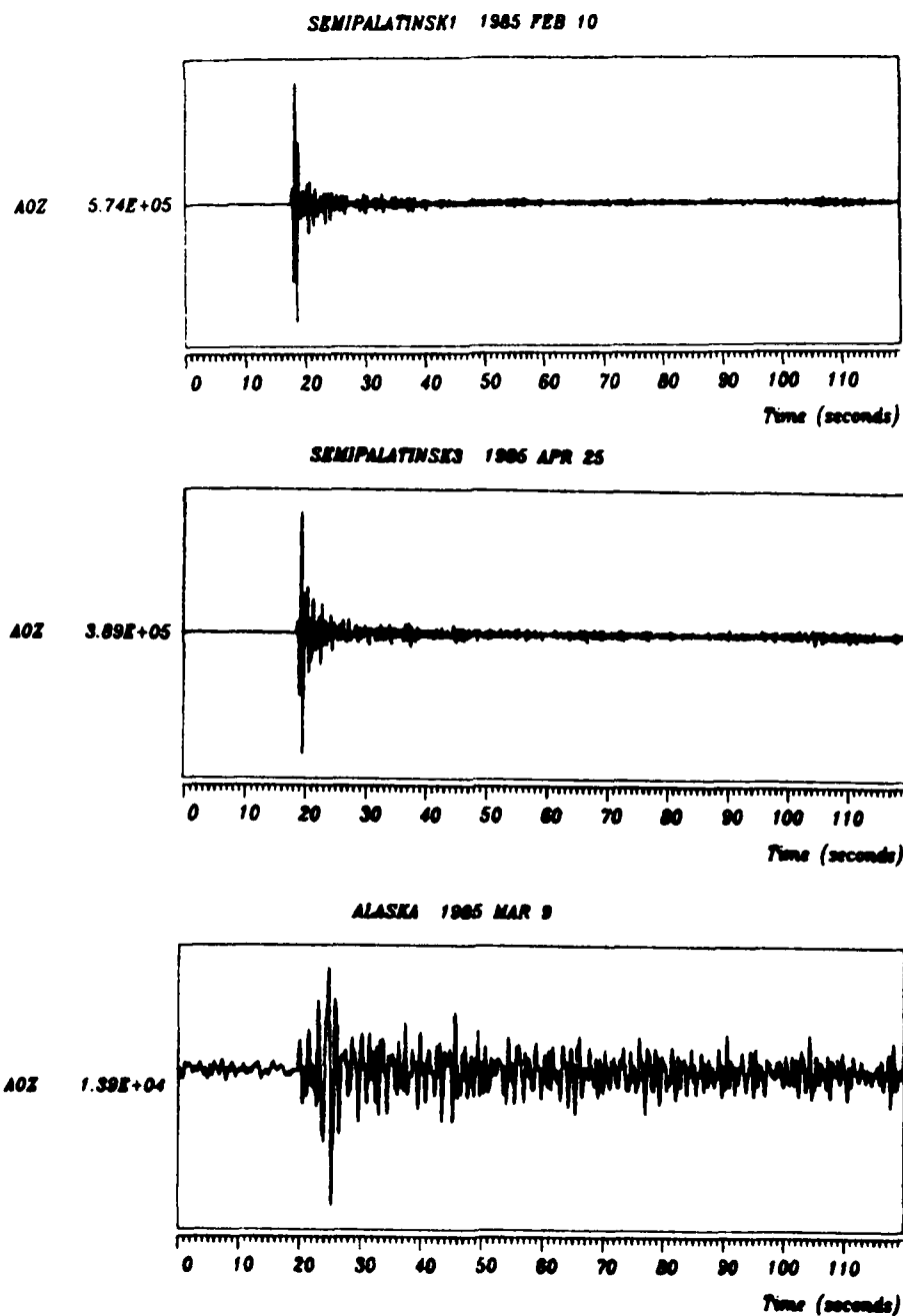
Figure 16a. Events analysed by f-k and wavenumber spectra, as recorded at the center seismometer, NORESS. Time zero is: for Semipalatinsk 1, 3:34:5 (U.T.); for Semipalatinsk 3, 1:4:10; for Alaska, 14:17:0. See Table 4 for further details.
