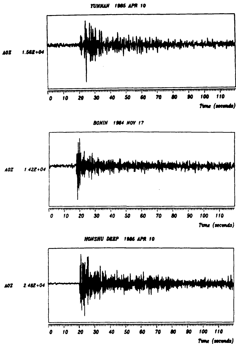
Figure 16b. Events analysed by f-k and wavenumber spectra, as recorded at the center seismometer, NORESS. Time zero is: for Yunnan, 6:3:35 (U.T.); for Bonin, 18:38:25; for Honshu, 16:37:25. See Table 4 for further details.
