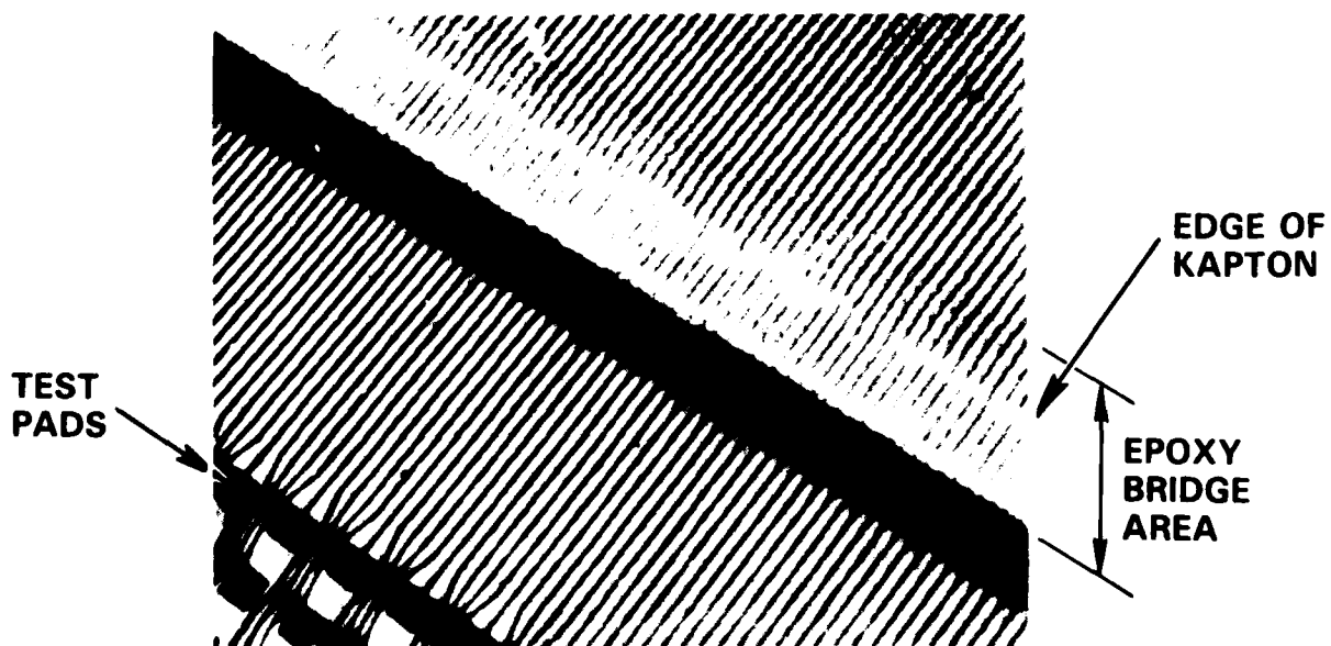
Fig. 7.4-2b Evaporated interconnect-enlarged view of (a) showing epoxy bridge over step edge of kapton.
