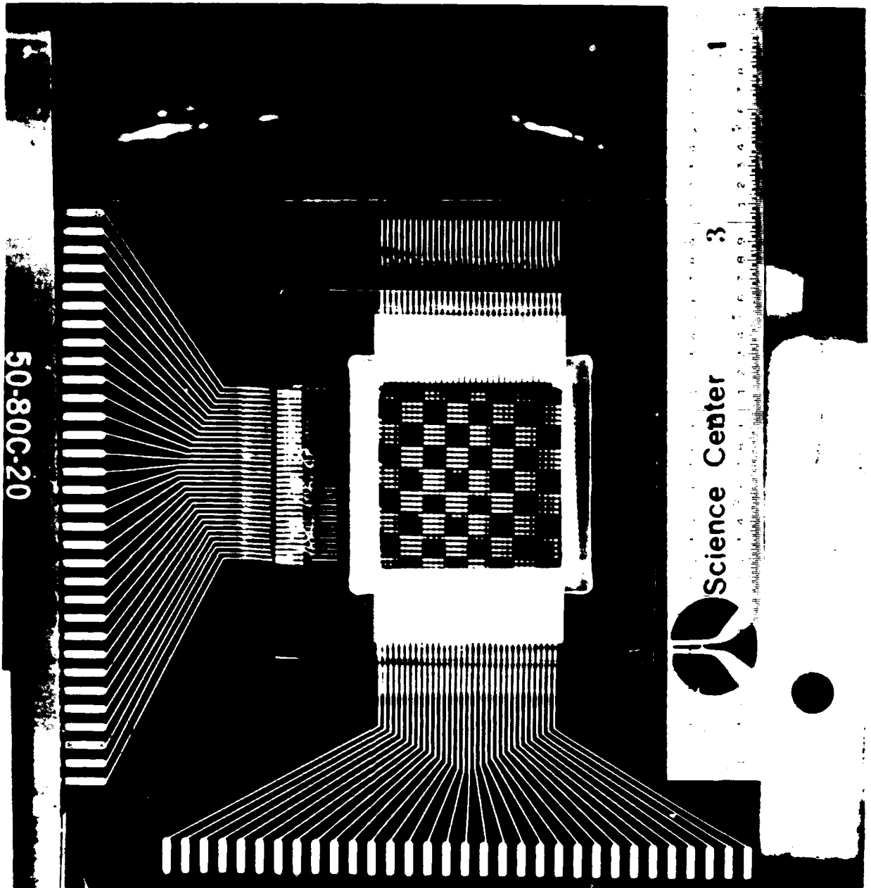
Fig. 4.3-1 Checkerboard pattern 32 x 32 display.
