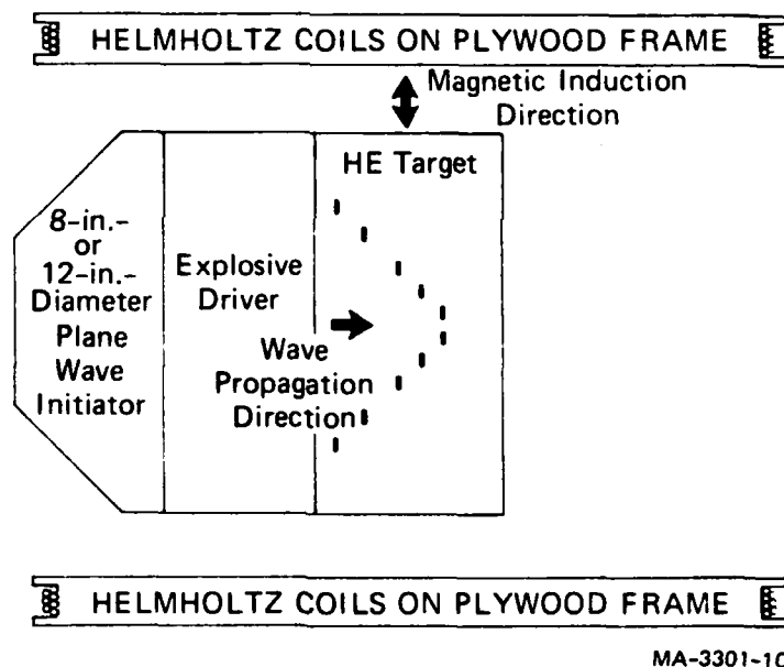
Figure 2. Configuration of SRI large-scale Lagrange particle velocity gage experiments. Heavy dashes in the HE target indicate the active elements of the embedded particle velocity gages.
