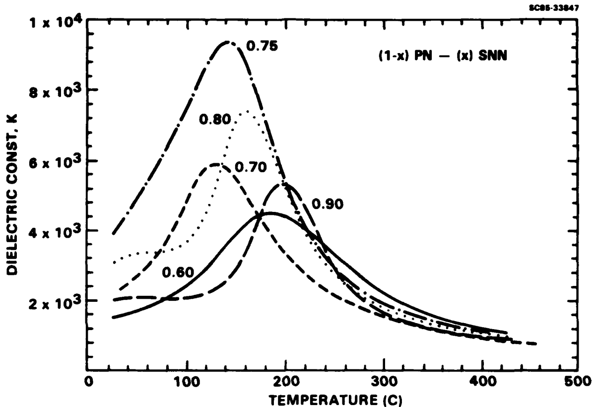
Fig. 17 Dielectric constant vs temperature for several PKN-SNN compositions. F = 10 kHz.
