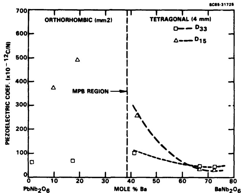
Fig. 12 Piezoelectric behavior of Pb_{1-x}Ba_xNb_2O_6 as a function of composition.
