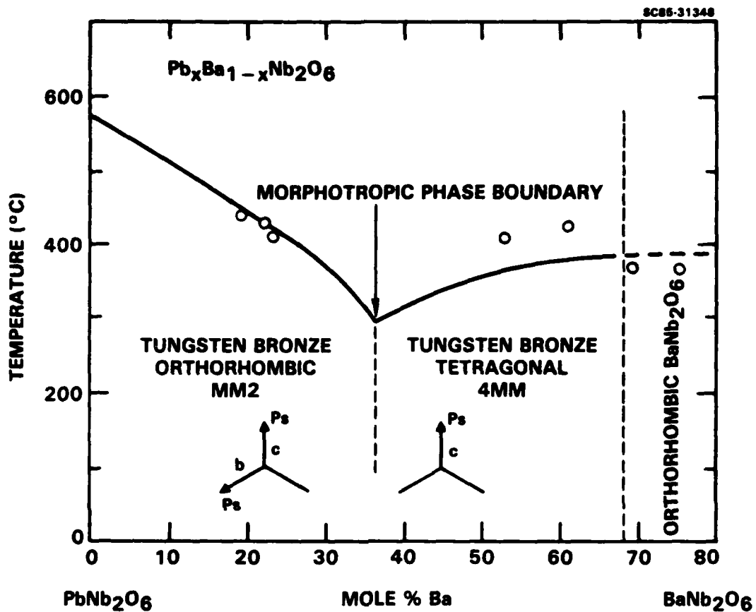
Figure 11 Phase diagram for the PbNb_2O_6 - BaNb_2O_6 system.
