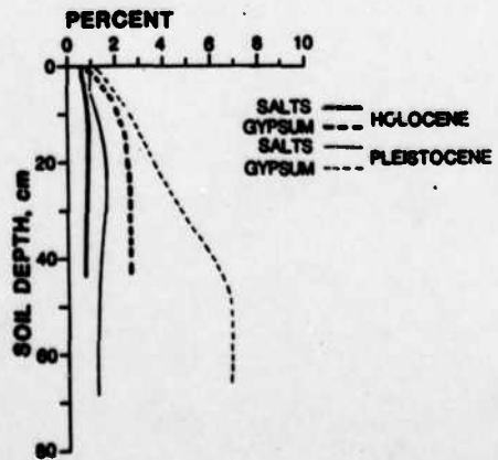
Figure C.1.23 The average content of salts and gypsum in various aridisols.
