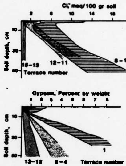
Figure C.3.6 Variation of gypsum and chlorides with depth, in a sequence of Holocene Reg soils (terrace no. 1 - oldest; terrace no.15 - youngest), Nahal Z'elim (Dead Sea).
