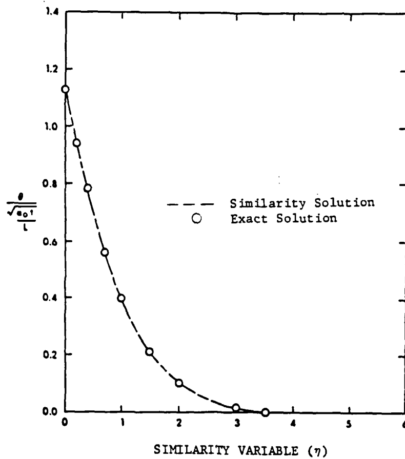
Figure 6. Temperature Distribution for Constant Properties (boundary condition Q_w = \text{constant} )
