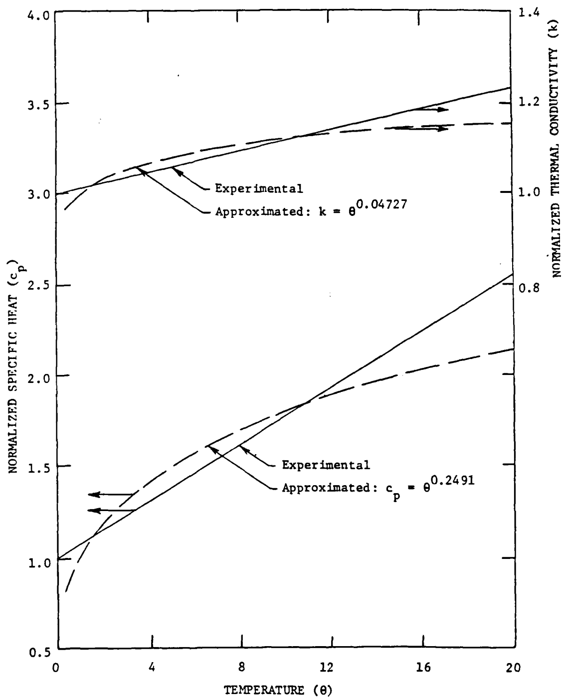
Figure 3. Thermal Properties of Type 420 Stainless Steel (normalized)
