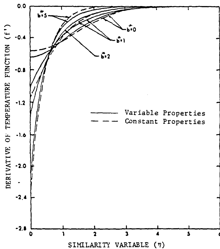
Figure 10. Profiles of Derivative of Temperature Function (boundary condition T_w = T_0(1 + t^{b^*}) )
