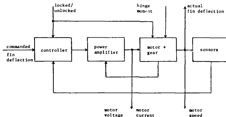
Fig B-2 Functional Block Diagram
