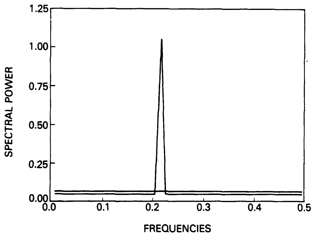
Fig. 2. Initial spectrum estimates P_{\mu\mu} (with peak) and P_{\sigma\sigma} (flat) for example.
