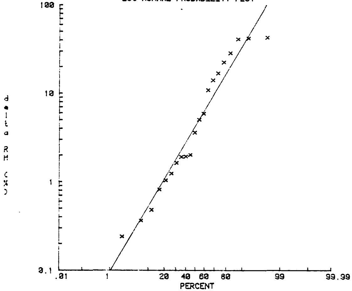
Fig 10 A log normal probability plot from the tethered balloon flights at 200 feet showing the differences between up and down measurements of relative humidity.
