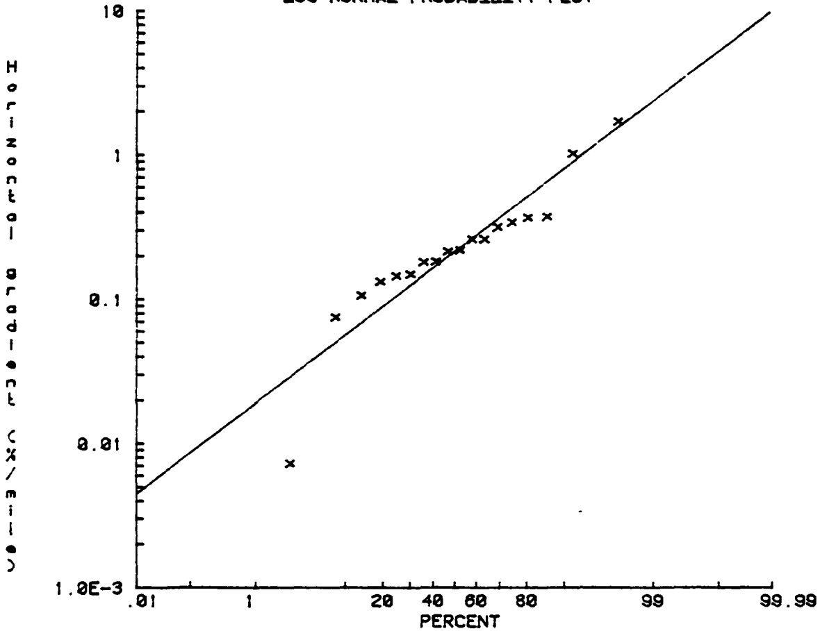
Fig 13 A log normal probability plot from the SNI tethered balloon flights at 2000 feet showing the estimated horizontal gradients in relative humidity.
