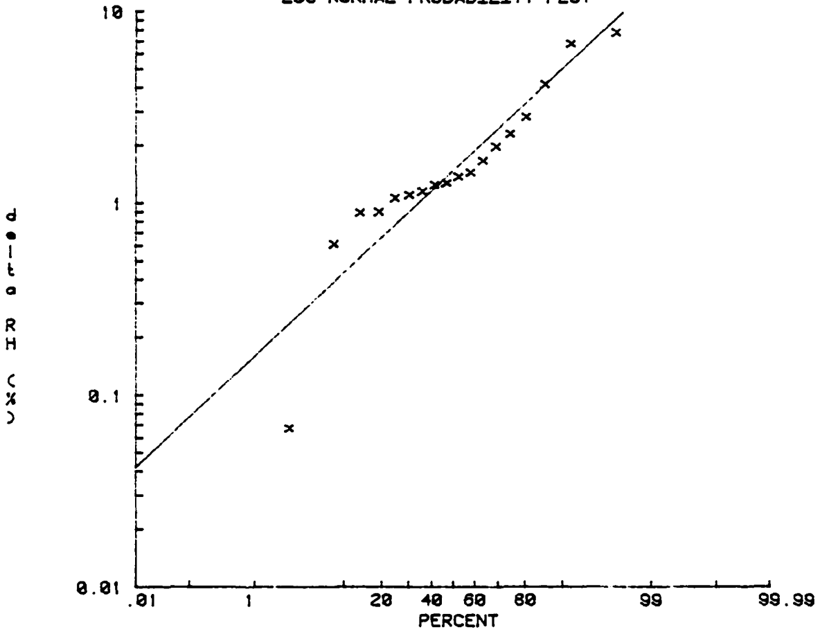
Fig 11 A log normal probability plot from the SNI tethered balloon flights at 2000 feet showing the differences between up and down measurements of relative humidity.
