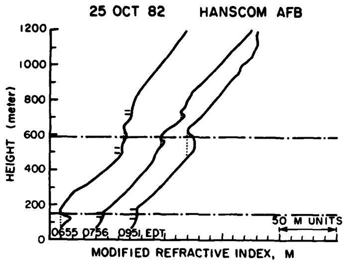
Figure 15. Modified Refractivity Profiles Measured at Hanscom AFB, 25 October 1982
