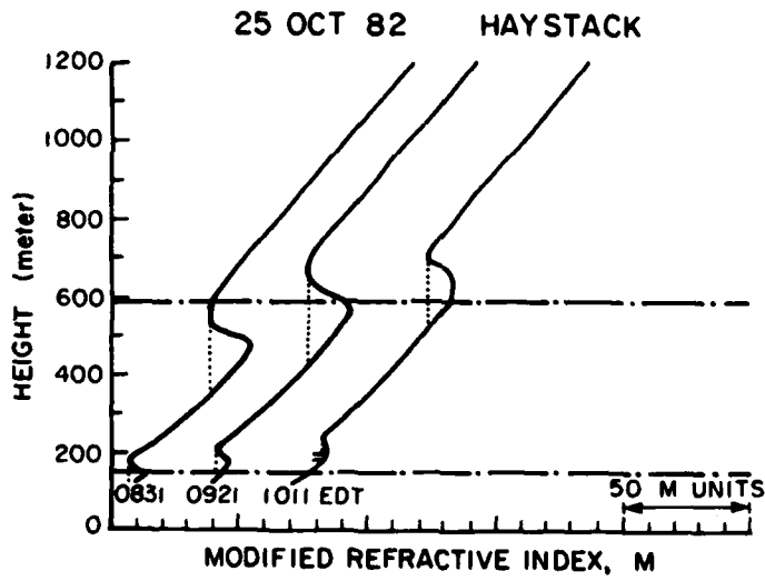
Figure 16. Modified Refractivity Profiles Measured at Haystack Site, 25 October 1982
