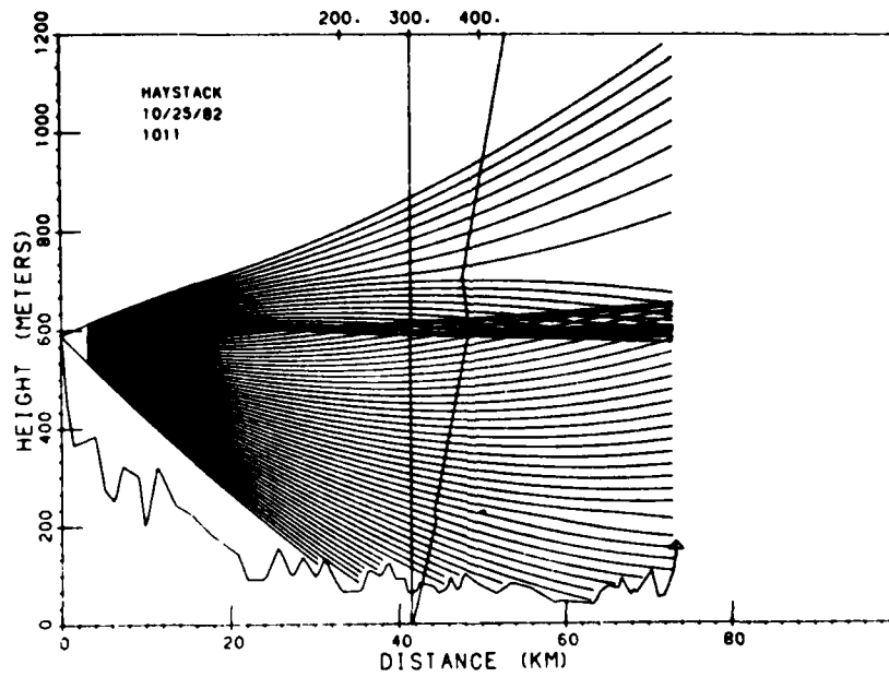
Figure 21. Ray Trace for Monadnock Link Using Sounding Data From Haystack Site at 1111 EDT, 25 October 1982
