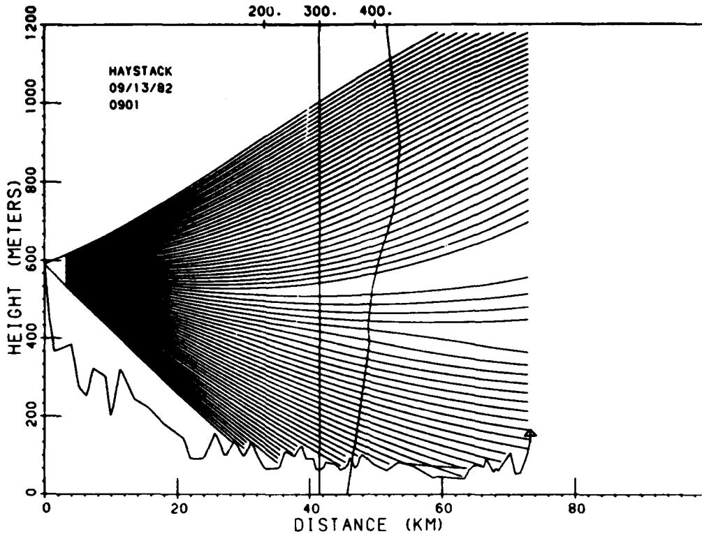
Figure 13. Ray Trace for Monadnock Link Using Modified Refractivity Profile From Haystack Sounding at 0901 EDT, 13 September 1982
