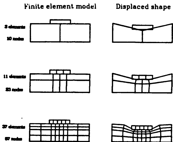
Figure 11: Rigid punch into an elastic foundation.
