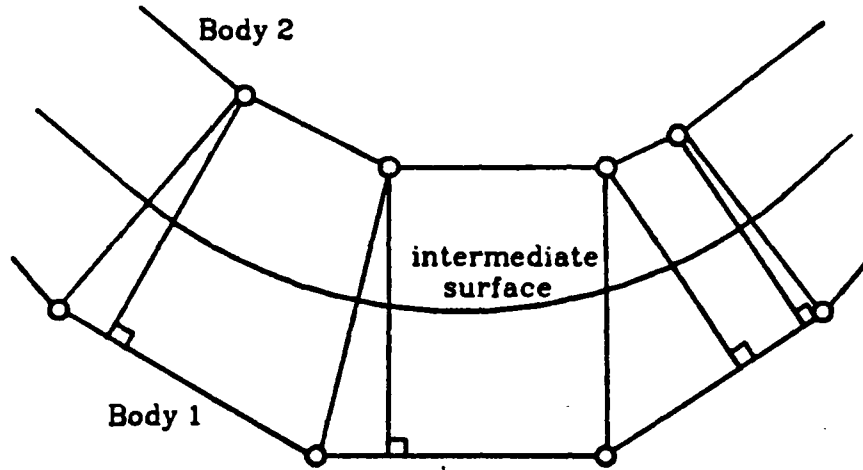
Figure 9: Possible problems with the slide line logic.
