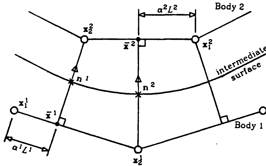
Figure 8: A typical contact segment.
