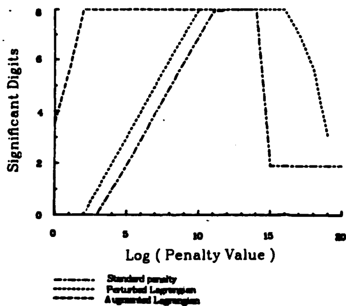
Figure 12: Results after 1 iteration for the 3 element mesh.
