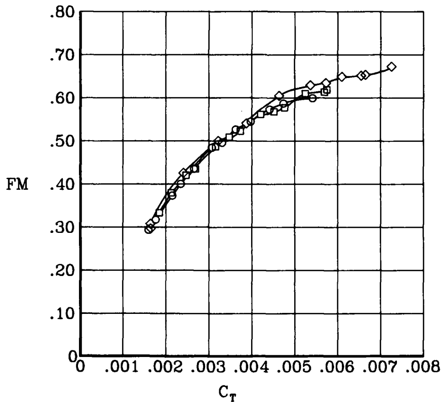
Figure 6. Comparison of aerodynamic characteristics of three rotors at two tip speeds.
