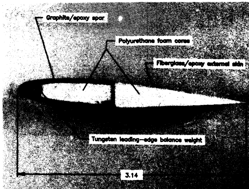
(c) Details of model rotor blade construction for TR3 platform.
