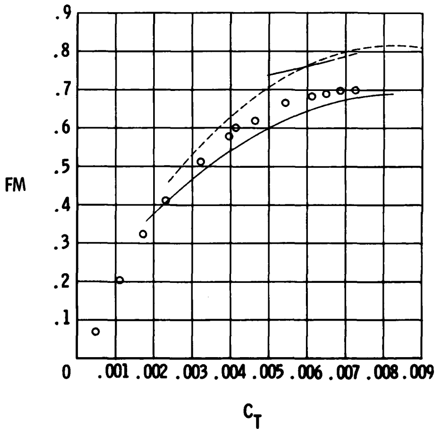
(b) TR3 planform.
