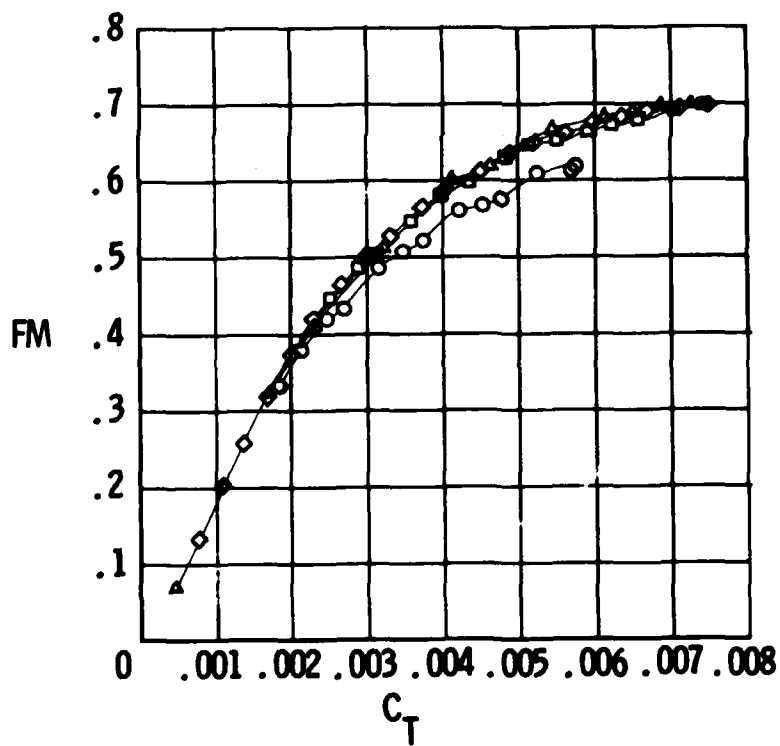
(b) TR3 platform.
