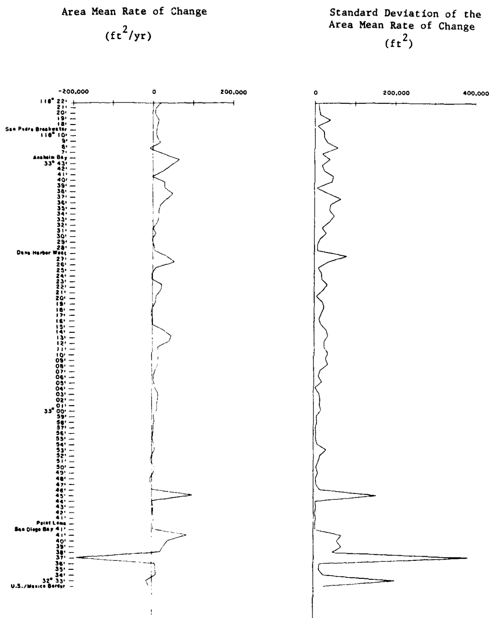
Figure 4. Area mean rate of change and standard deviation, maximum available survey record ( \geq 1852 - 1982 )
