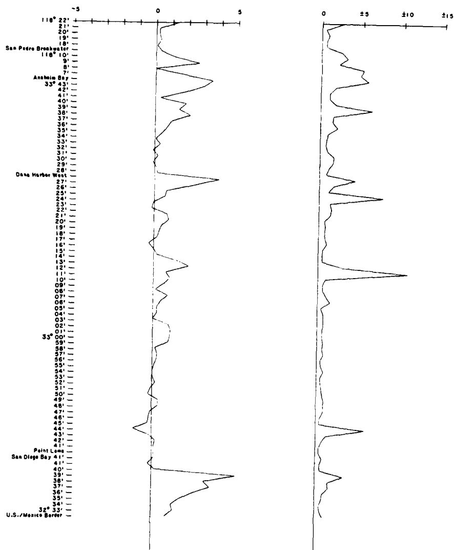
Figure 6. Shoreline mean rate of change and standard deviation, maximum available survey record ( \geq 1852 - 1982 )
