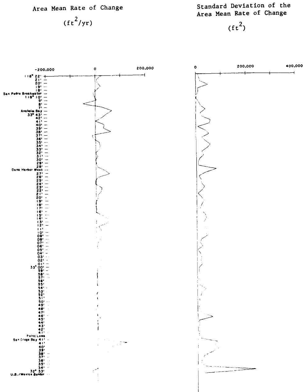
Figure 5. Area mean rate of change and standard deviation, maximum available survey record (≥1933 - 1982)
