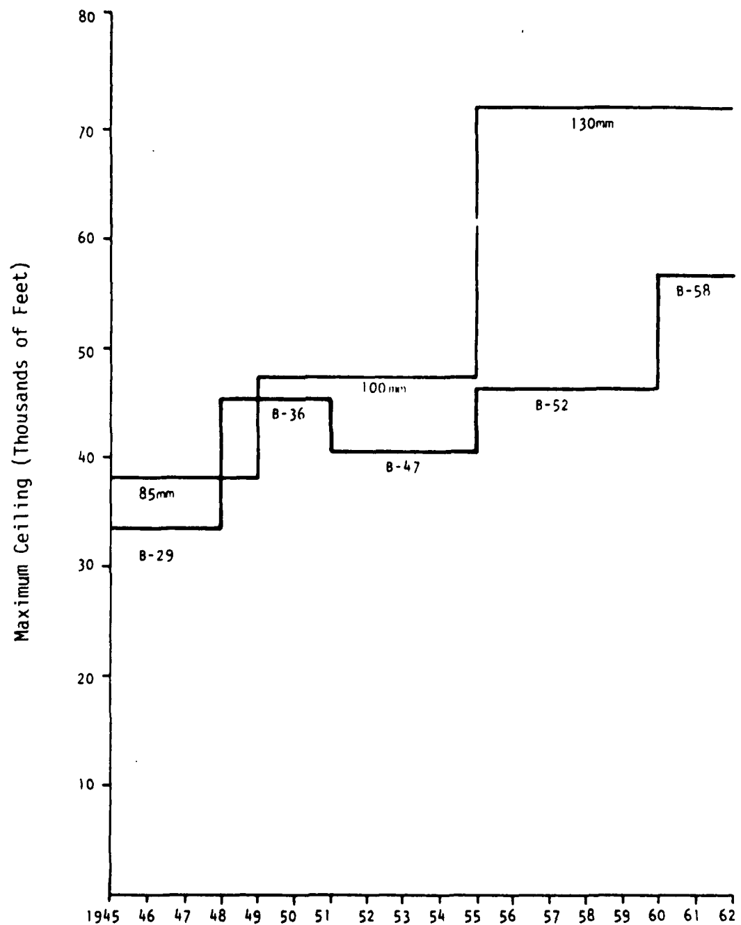
Altitude Capabilities of AAA and Bombers since World War II
