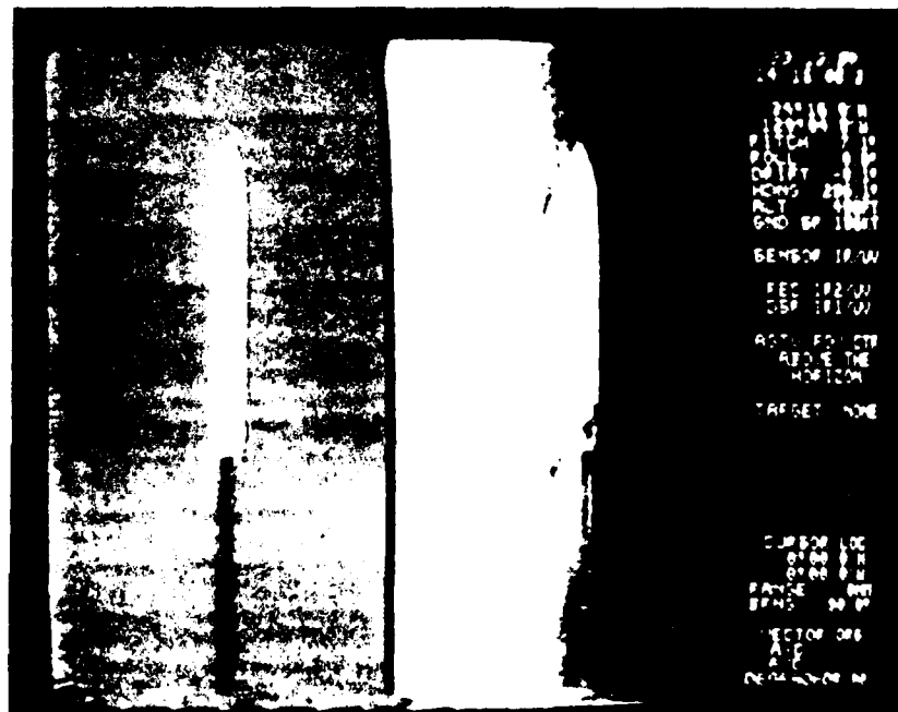
Figure 3-22. Run 7, 9/13/84, 14:15, Altitude 500 Feet. Photograph of stop frame of video screen showing low altitude image of container ship (IR on left, UV on right).
