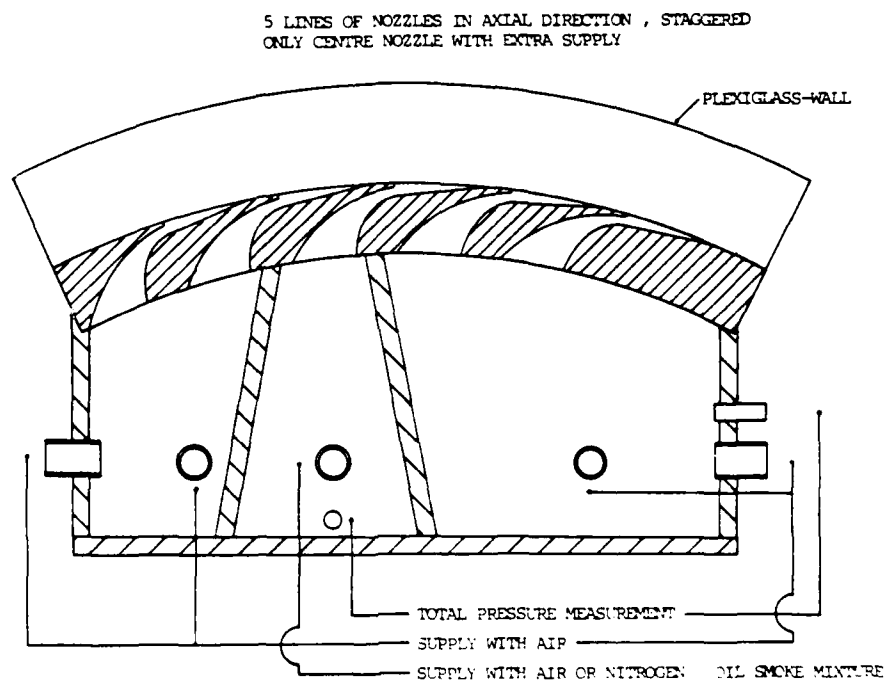
Figure 4 : 25 Jets Flow Model
