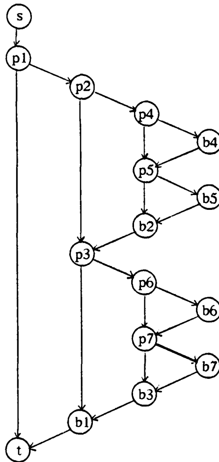
Figure IX-3. Flowgraph INA with n = 7 predicates
