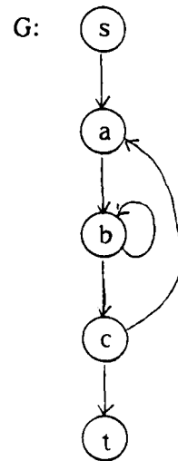
Figure IV-3. A finite subset that is not loop adequate
