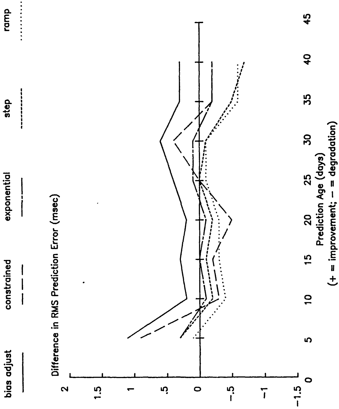
Figure 5: Change in UT1-UTC Predictions (compared with "production" solutions)
