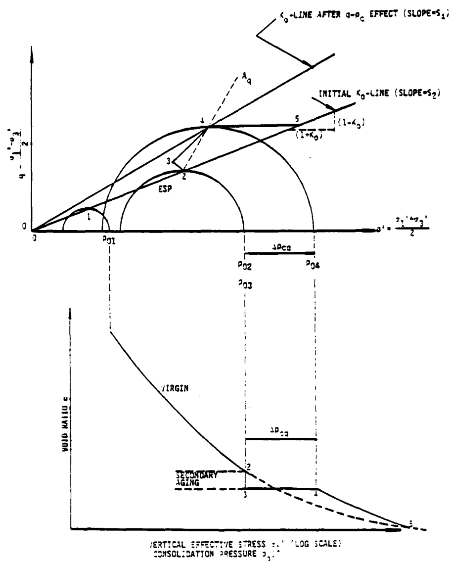
Figure 2-1 Effective Stress Path (ESP) before, during, and after the q-p_c effect (Modified after Schmertmann, 1981, p. 479)
