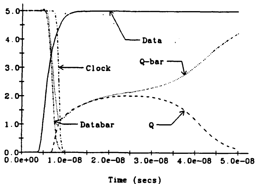
Figure A.3: SPICE2.G5 Simulation of the CMOS Bistable Latch
