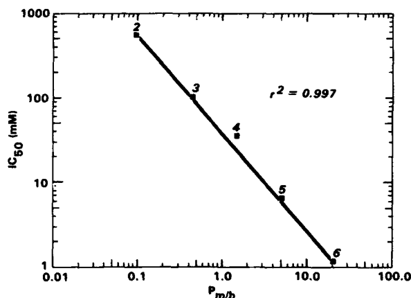
Fig. 6. Correlation of the inhibitory potency of aliphatic alcohols on BTX-stimulated ^{22}\text{Na}^+ uptake with their membrane/buffer partition ( P_m/b ) coefficient. The concentration of each alcohol that inhibits BTX-stimulated ^{22}\text{Na}^+ uptake by 50% ( \text{IC}_{50} , millimolar) is presented on the ordinate. The P_m/b s are shown on the abscissa. The number above each symbol represents the chain length of the alcohol: 2, ethanol; 3, n -propanol; 4, n -butanol; 5, n -pentanol; and 6, n -hexanol. The line was fit by linear regression analysis with a correlation coefficient, r^2 = 0.997 . See table 3 for details.
