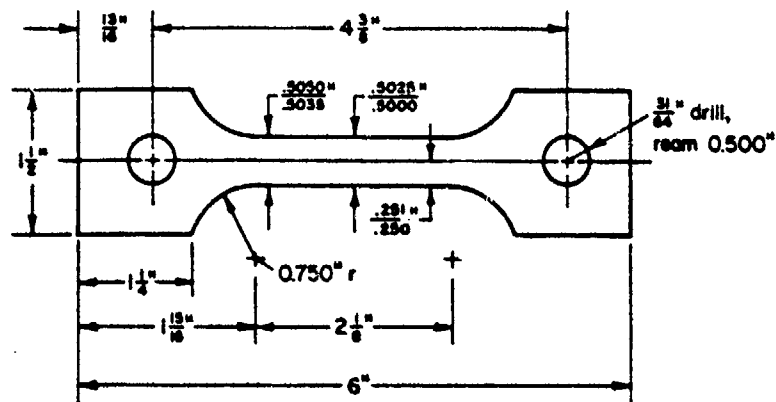
Figure B-20. Tensile specimen for Inconel 718 sheet.
