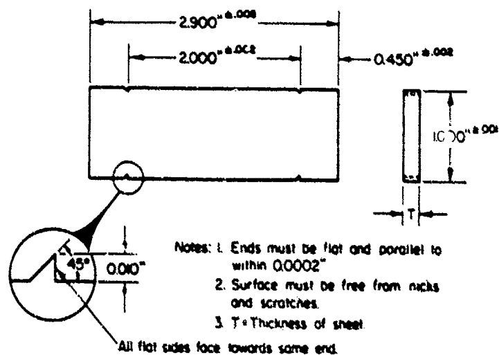
Figure B-21. Compression specimen for Inconel 718 sheet.
