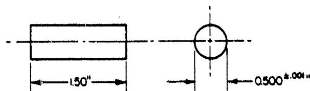
Figure B-3. Compression specimen for 7149-T73 hand forging.
