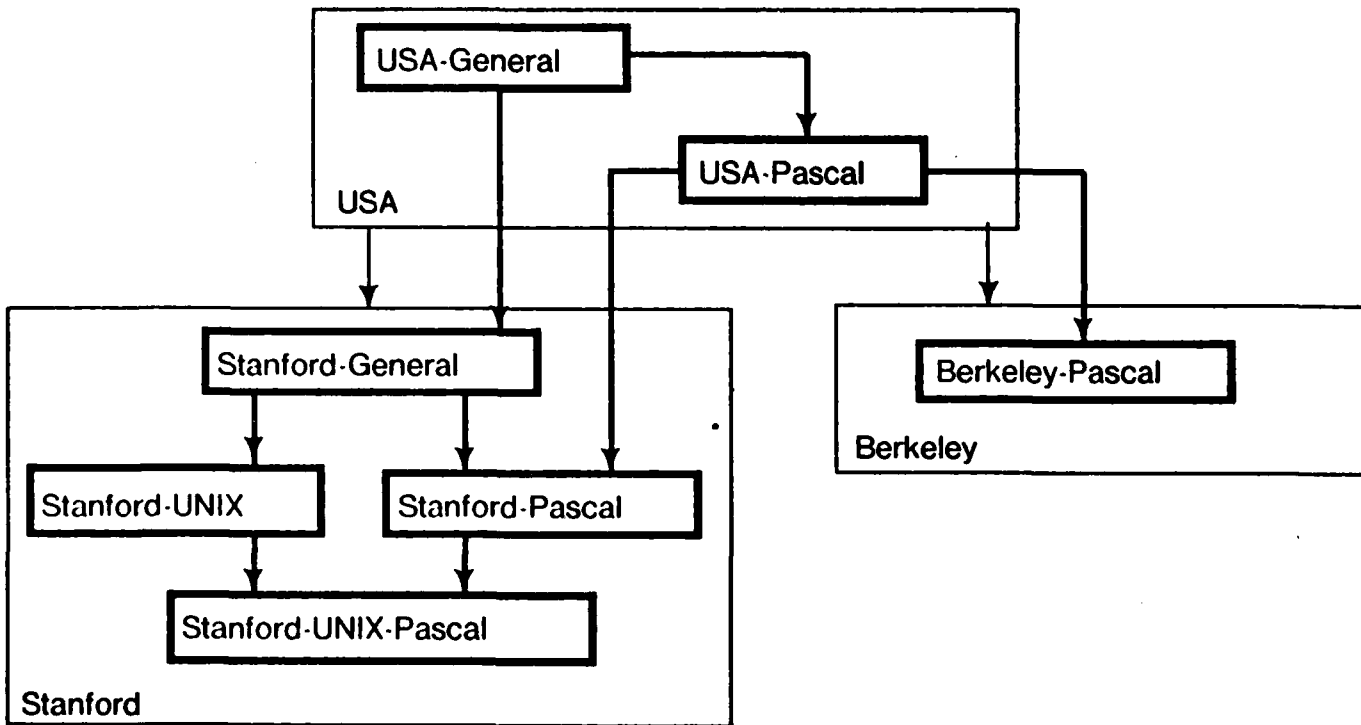
Figure 3-1: Example of a name space graph.
