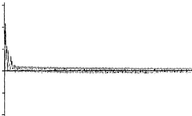
Fig. 25. Example 2 structure displacement/time K=6
