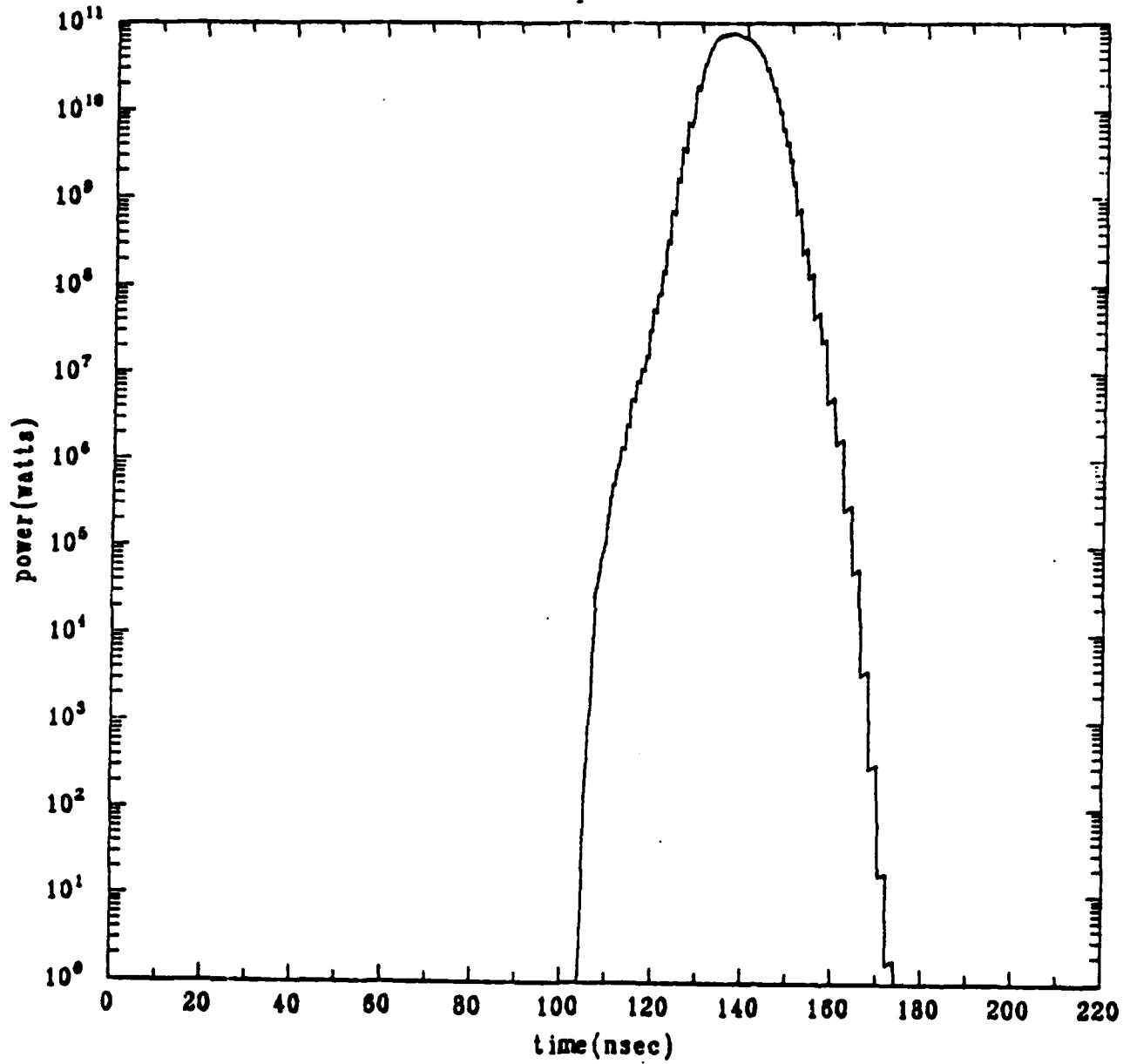
Fig. 9. Power radiated in heliumlike sodium resonance line as a function of time.
