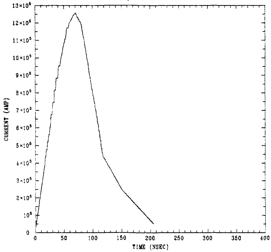
Fig. 1. Current waveform as a function of time.
