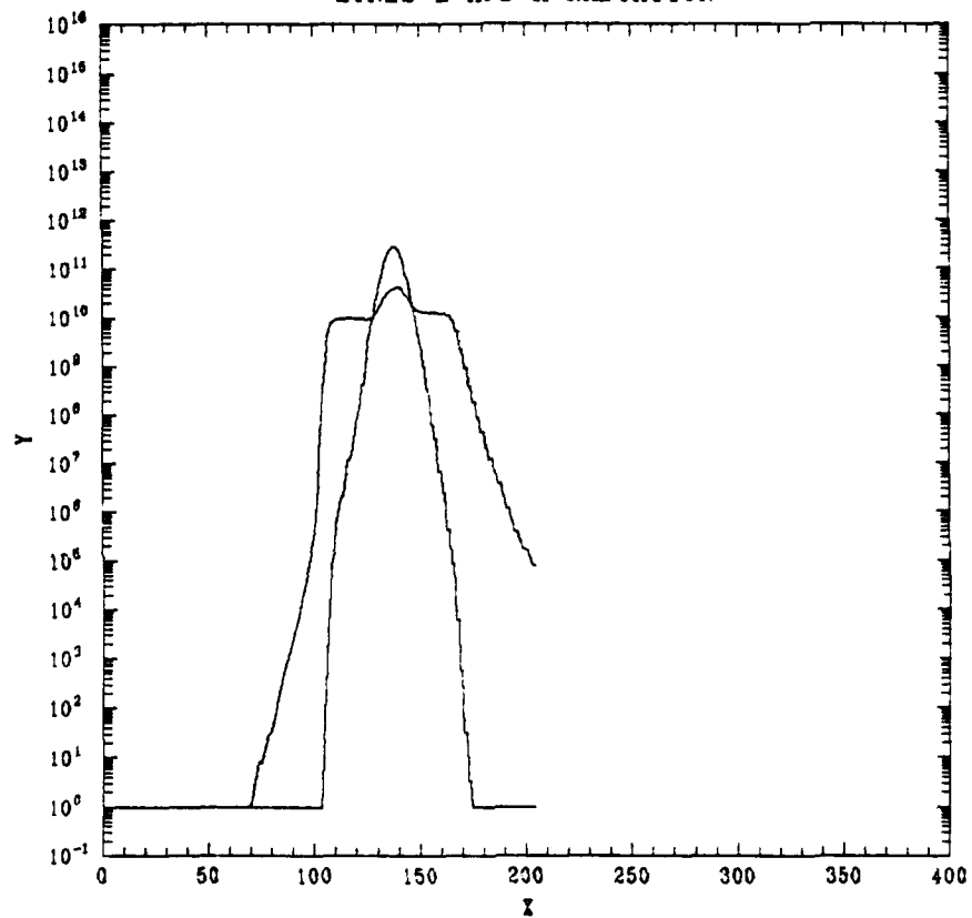
Fig. 7. Power radiated in L-and K-lines as a function of time.
