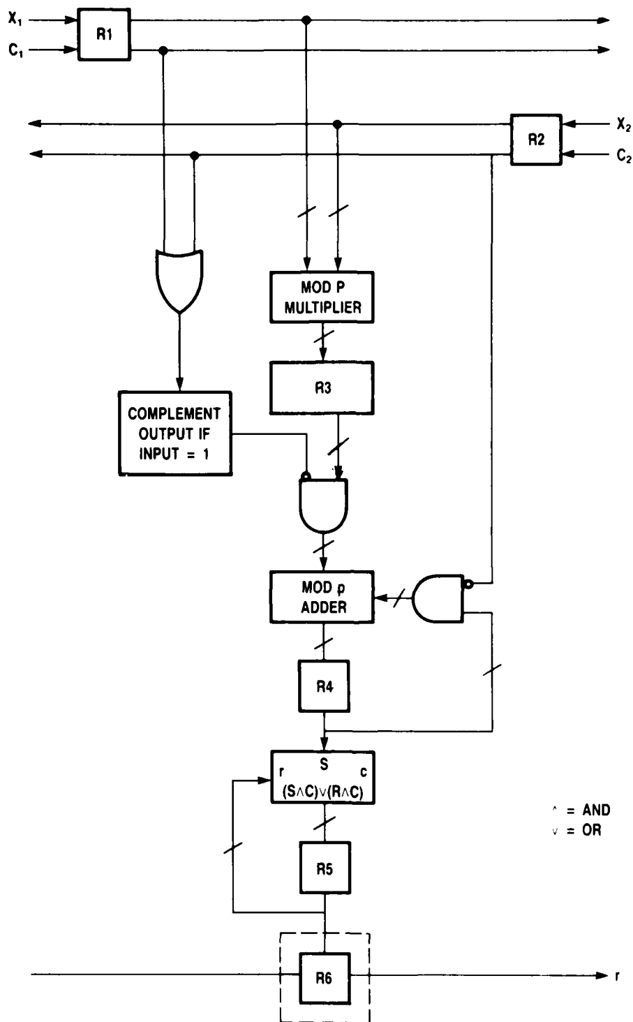
Figure 4.9. SYSTOLIC CORRELATOR CELL MOD p
