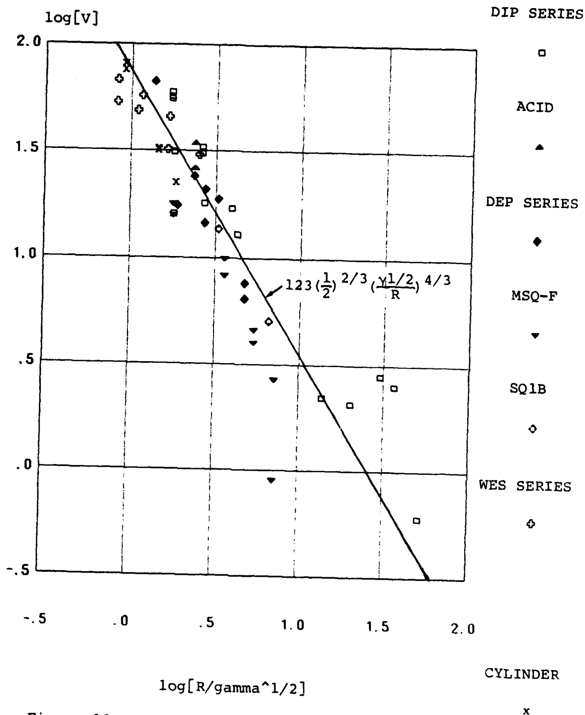
Figure 13. Cylindrical velocity attenuation.
