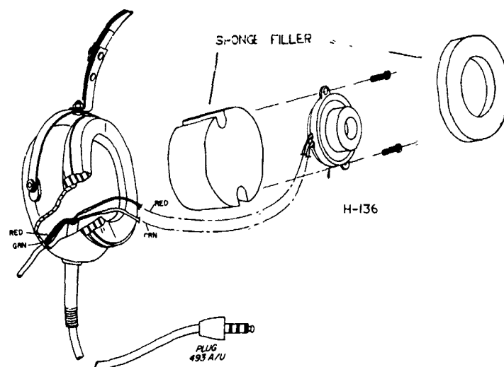
FIGURE 1 AN EXPLODED VIEW OF AN H-133 HEADSET EARCUP SHOWING THE SPONGE FILLER INSERTS, THE H-136 EARPHONE AND THE RED AND GREEN WIRES
