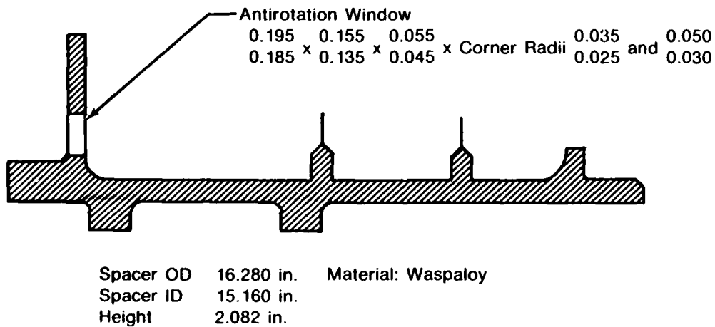
Figure H-13. 6-7 Compressor Spacer (P/N 4039846)
