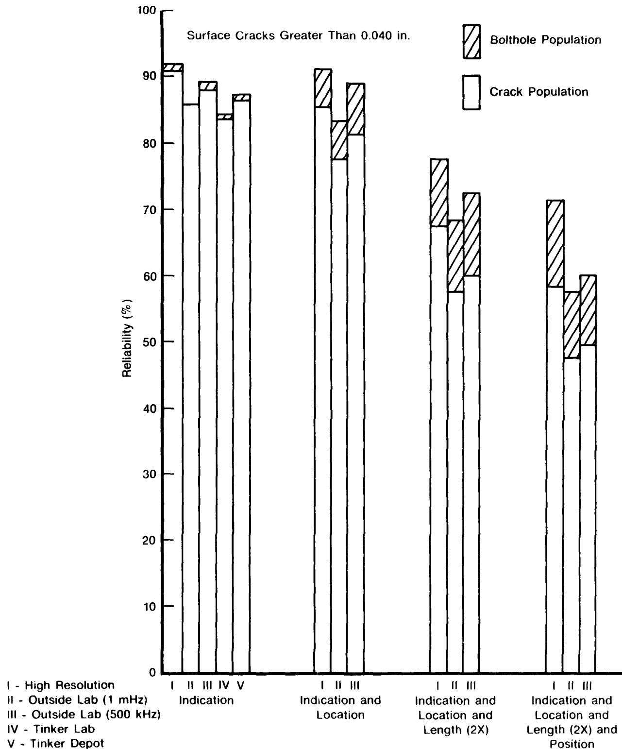
Figure J-10. Inspection Reliability of Detecting Cracks Greater Than 0.040 in. in Surface Length as a Function of the Various Agreement Criteria. Open Bars Are for a Crack Population Basis and Shaded Bars Are for a Bolthole Population Basis. (Figure from Failure Analysis Associates)
