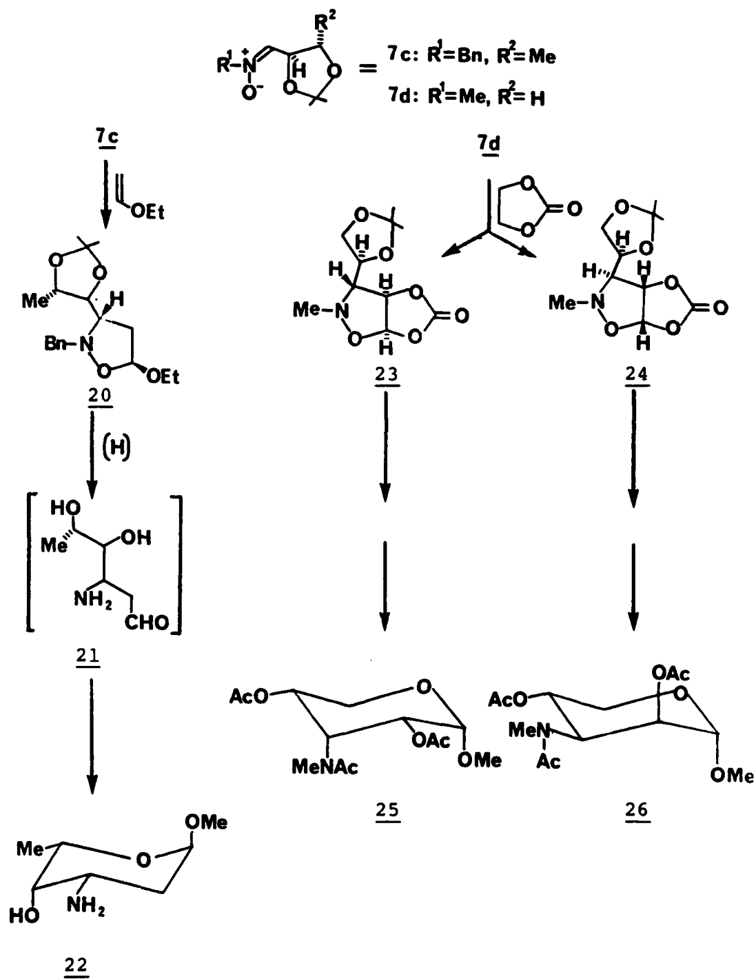
Scheme 10
