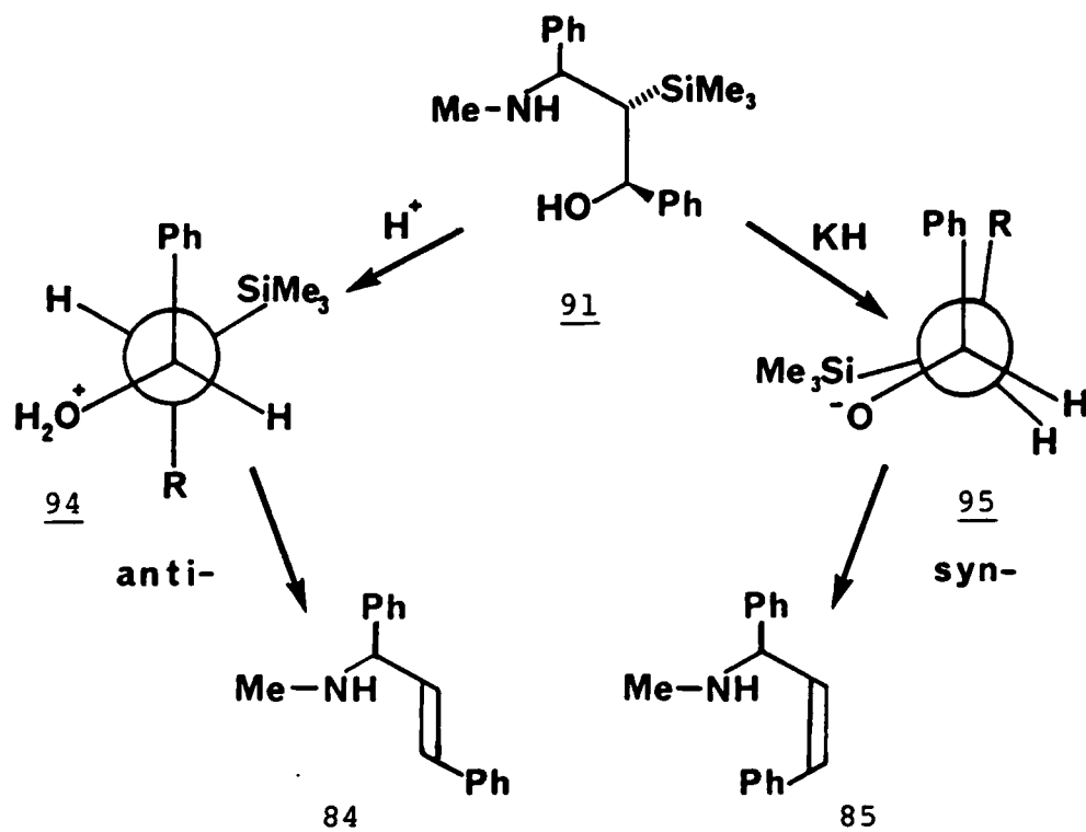
Scheme 25
