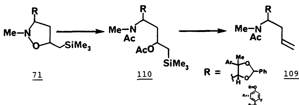
Scheme 31
