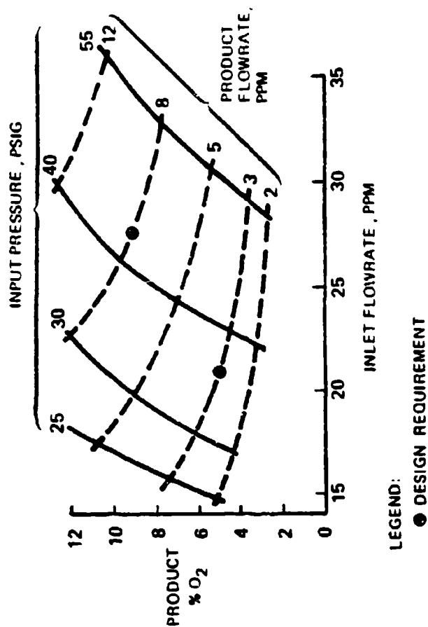
Figure 17. MSIGG Basic Performance at 75° F, Sea Level
