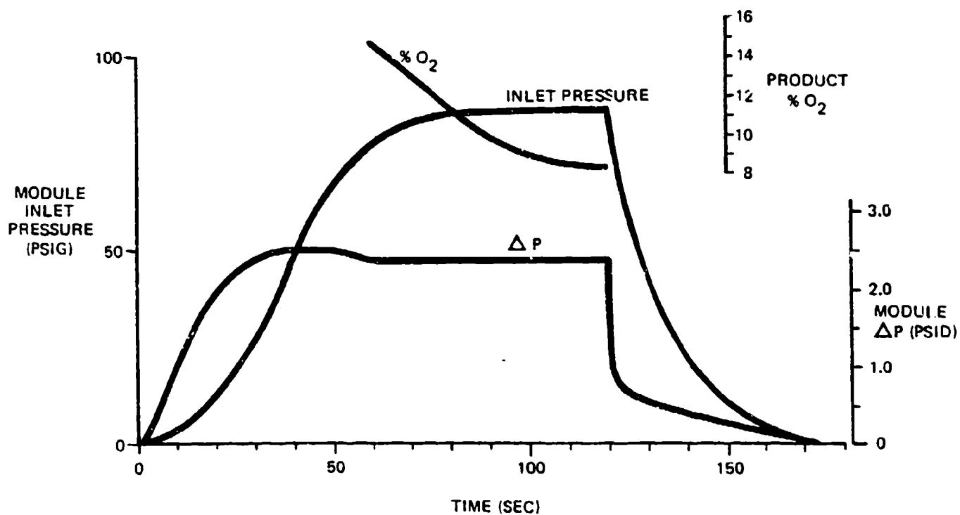
Figure 31. PMIGG "Soft Start" Cycle
