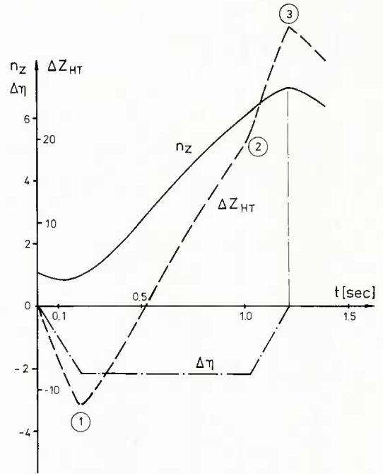
FIG. 3 LOAD FACTOR AND HORIZONTAL TAILPLANE LOADS FOR AN A/C WITH DIRECT SURFACE CONTROL
