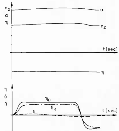
FIG. 16 ROLLING PULL OUT PARAMETERS FOR AN A/C WITH CSAS
