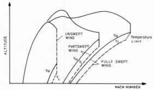
FIG. 9 FLIGHT ENVELOPE FOR VARIABLE WING SWEEP A/C
