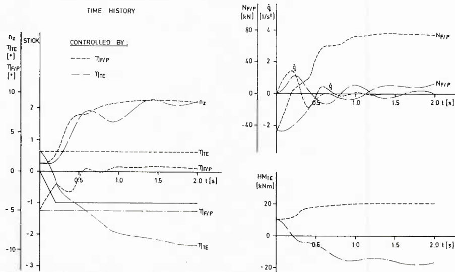
FIG 22 MOVEMENT AND LOADS OF CONTROL SURFACES CONTROLLED BY FOREPLANE OR TRAILING EDGE FLAP
