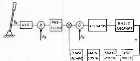
FIG. 11 CONTROL AND STABILITY AUGMENTATION SYSTEM OF SUPERSONIC AIRCRAFT
