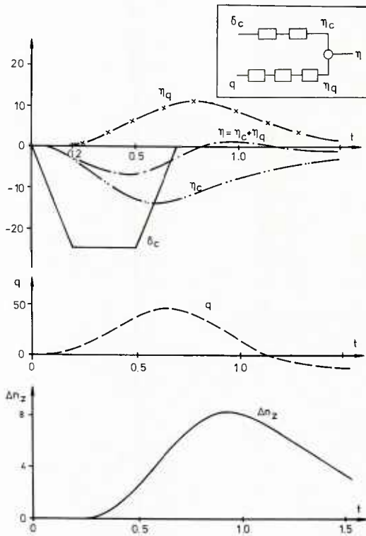
FIG. 6 DIFFERENCE BETWEEN COCKPIT CONTROL AND ELEVATOR DEFLECTION TIME HISTORY
