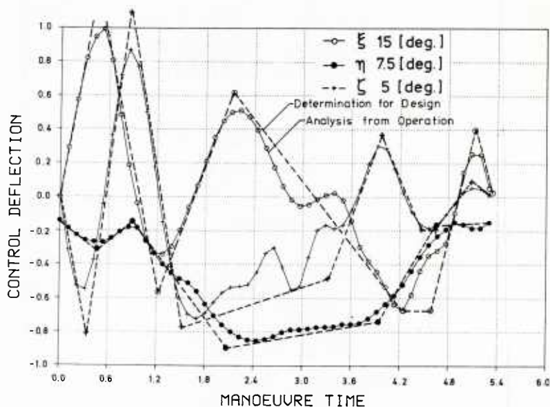
FIG. 25 EXTREME OPERATIONAL CONTROL SURFACE DEFLECTIONS (HIGH-6-TURN)
