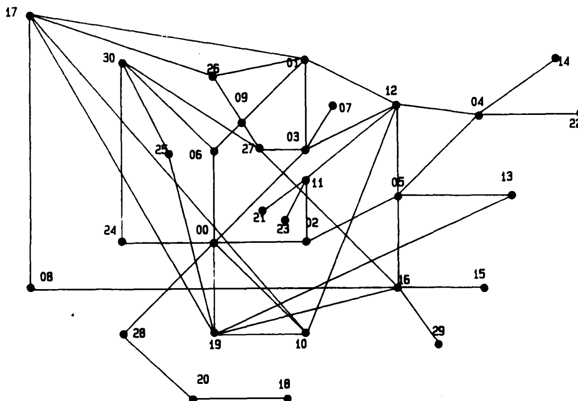
Configuration N3103 31 Nodes, 48 links Randomly Generated Network
