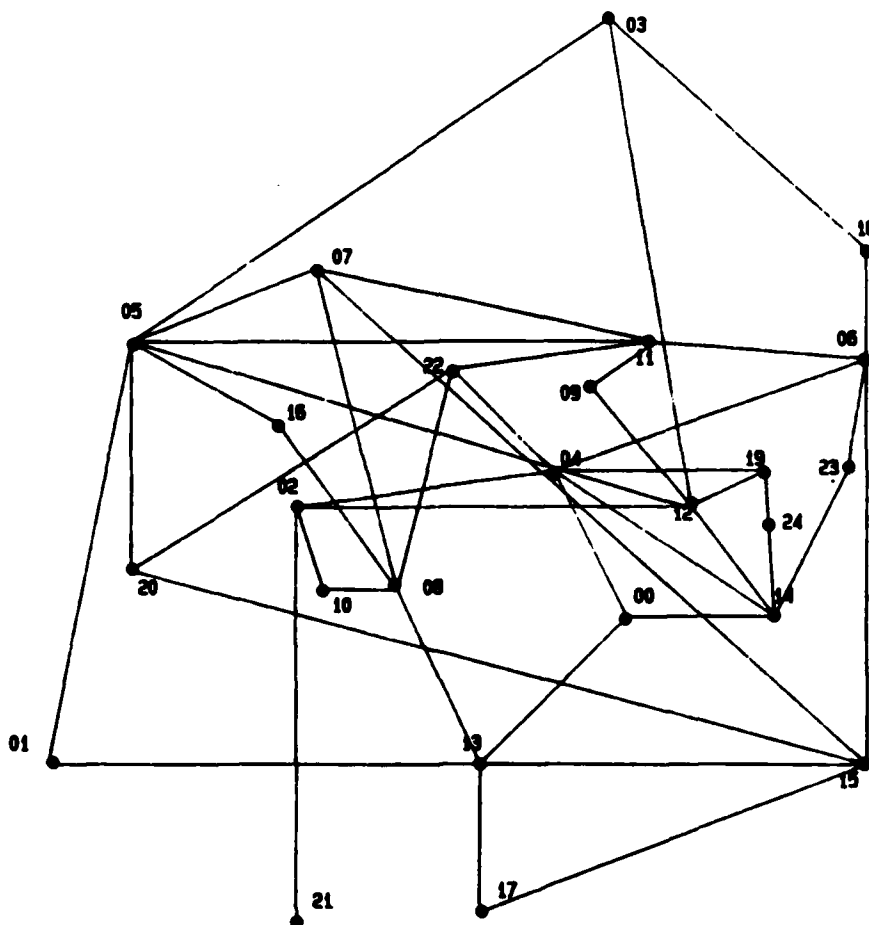
Configuration N2501 25 Nodes, 46 links Randomly Generated Network
