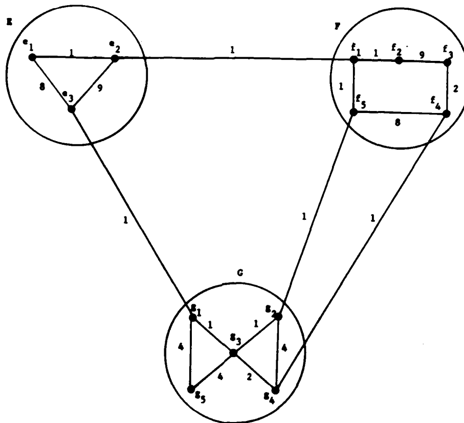
Figure 3-1. Area Routing Example
