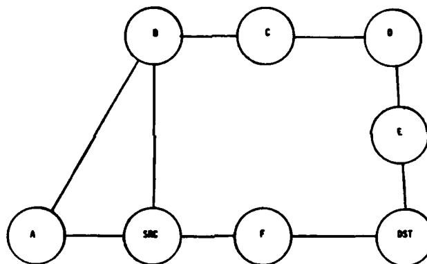
Network Configuration with Possible Routing Loops
