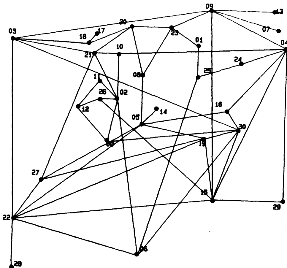
Configuration N3102 31 Nodes, 55 links Randomly Generated Network
