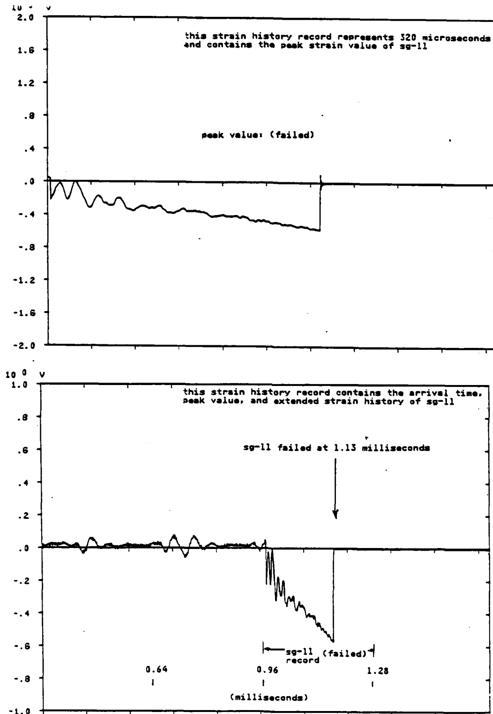
Figure 4.37 Strain Gage NO. 11 Strain History.
