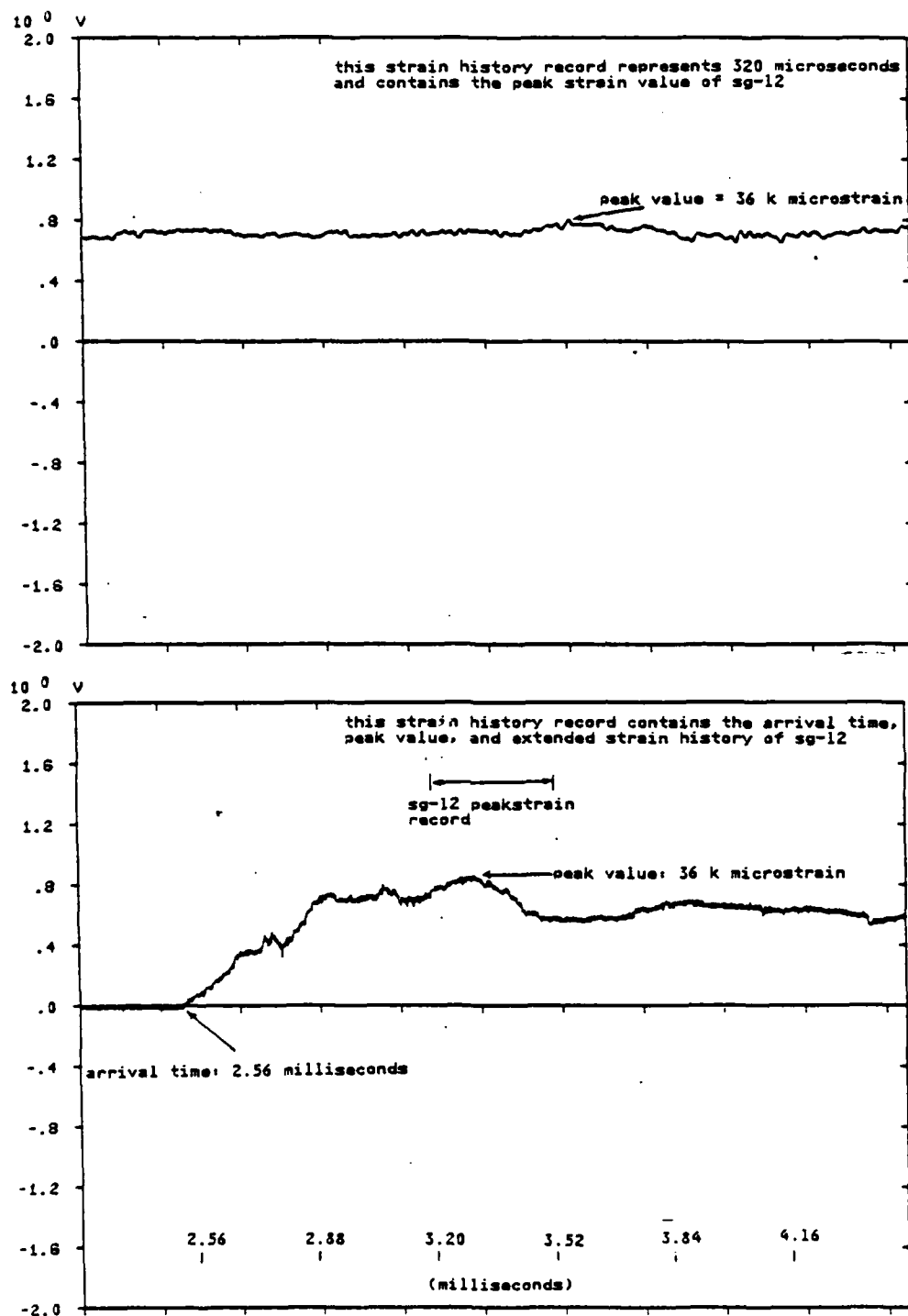
Figure 4.38 Strain Gage NO. 12 Strain History.
