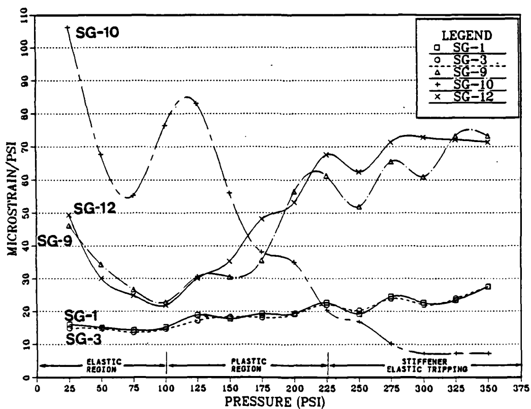
Figure 4.18 Plot of Static Strain Normalized to Pressure.
