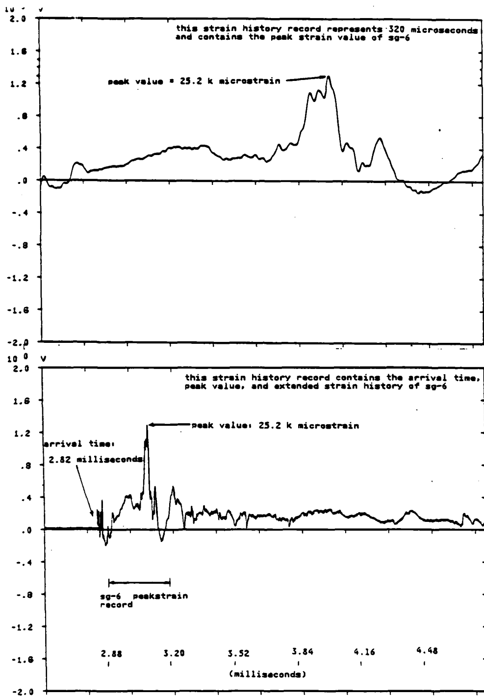
Figure 4.32 Strain Gage NO. 6 Strain History.
