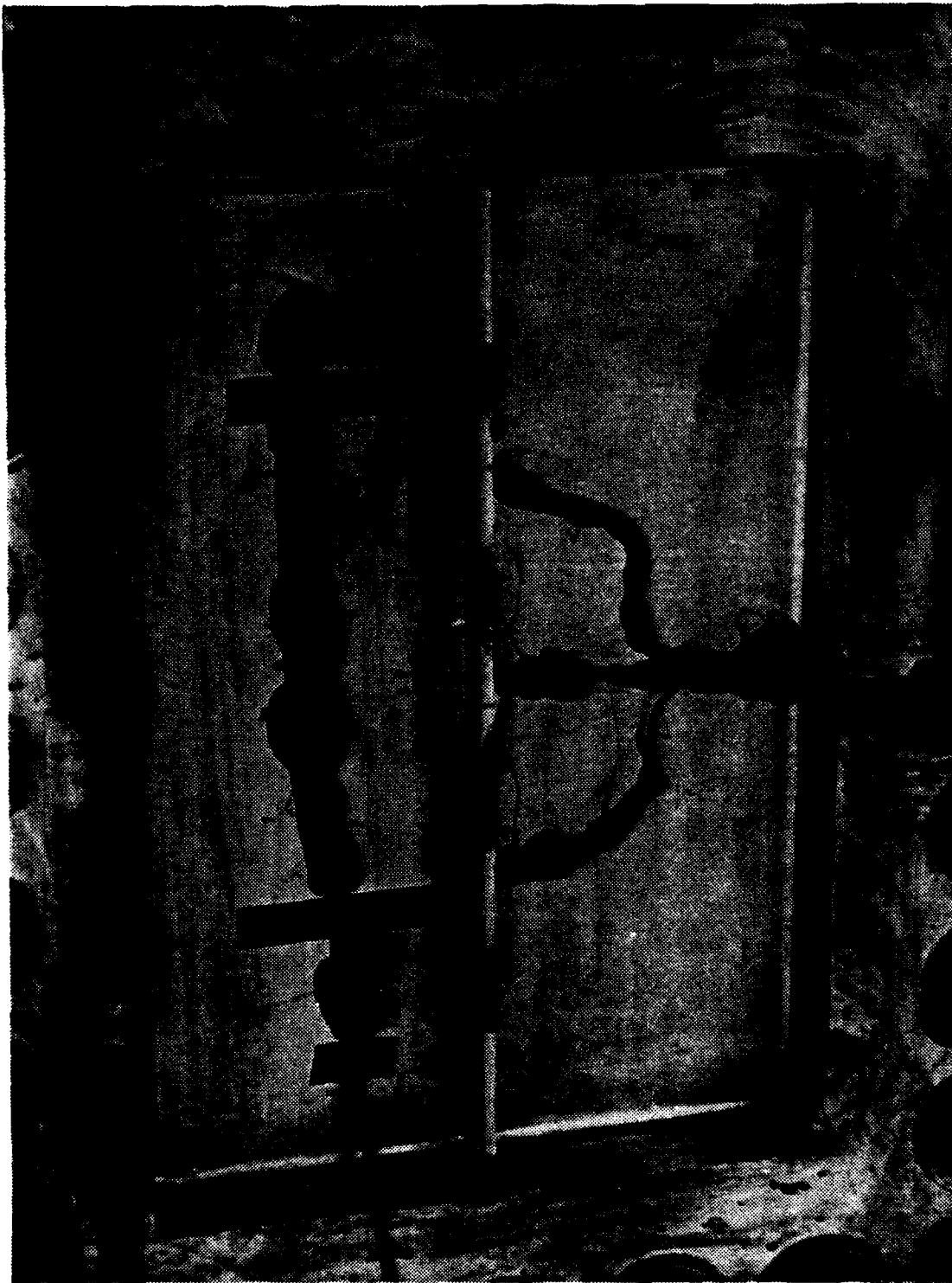
Figure 3.7 Strain Gage and Pressure Transducer Placement (waterside).
