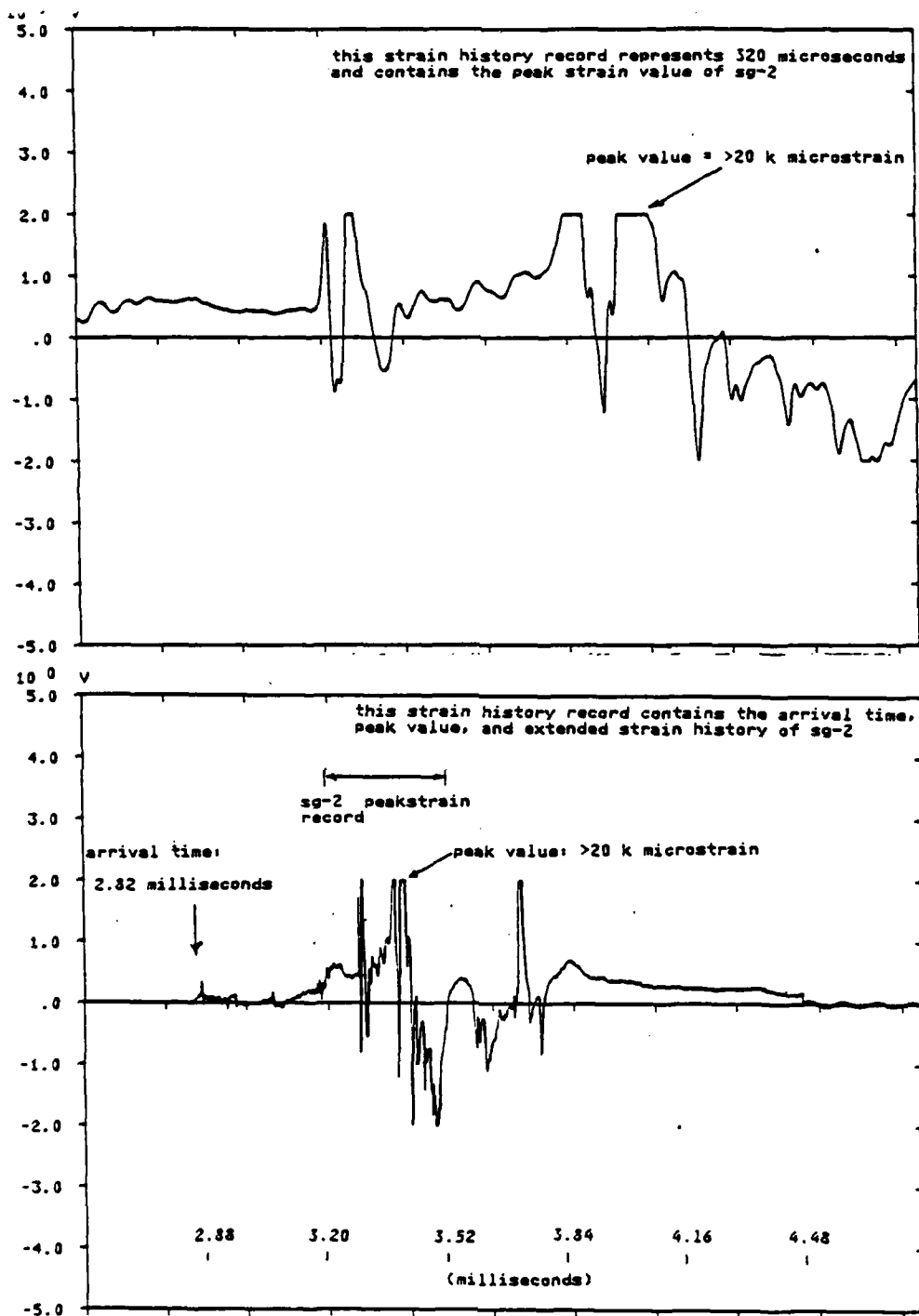
Figure 4.28 Strain Gage NO. 2 Strain History.
