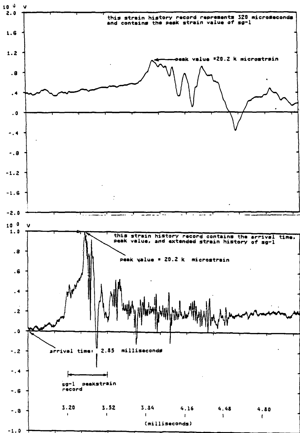
Figure 4.27 Strain Gage NO.1 Strain History.
