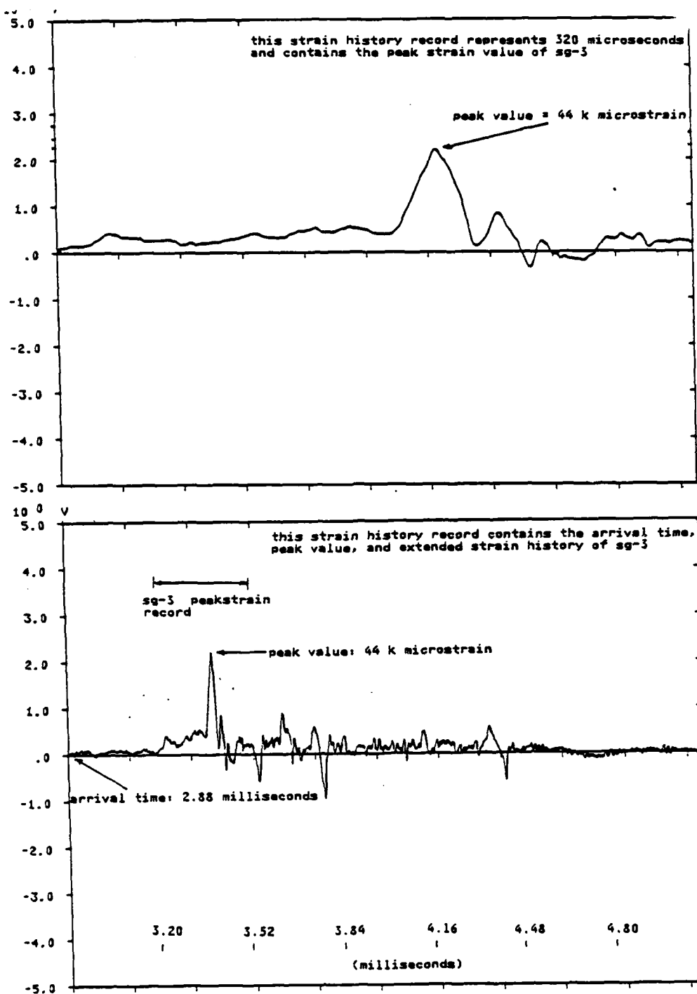
Figure 4.29 Strain Gage NO. 3 Strain History.
