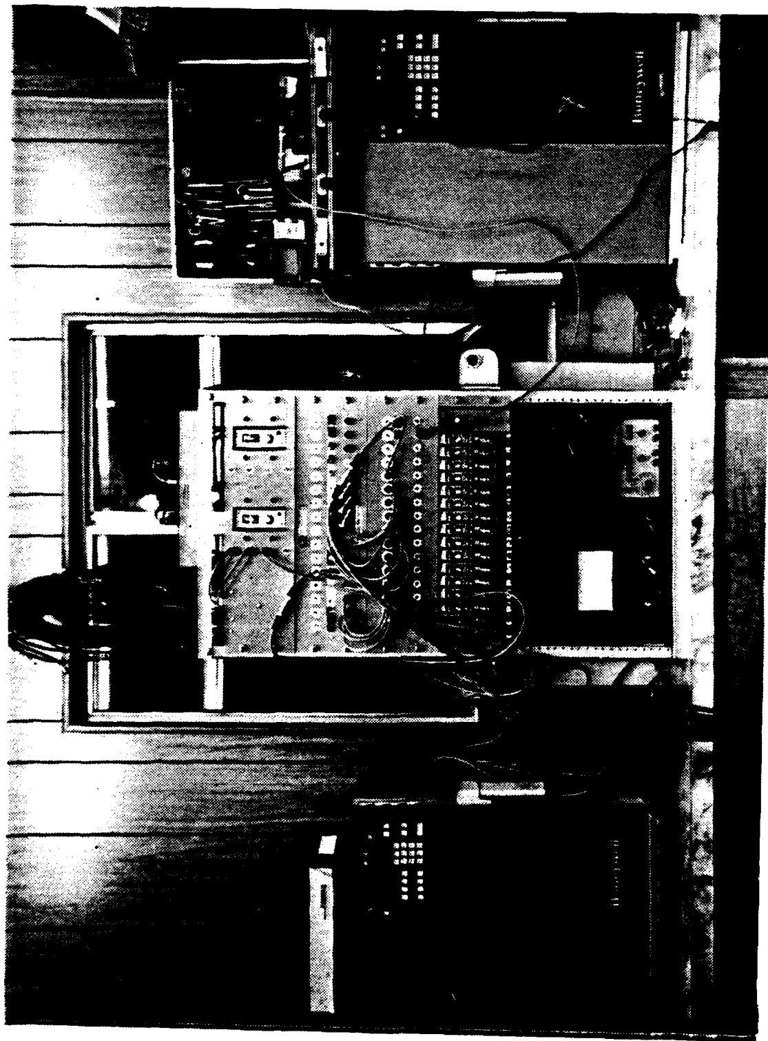
Figure 3.10 Undex Data Recording Instrumentation Arrangement.
