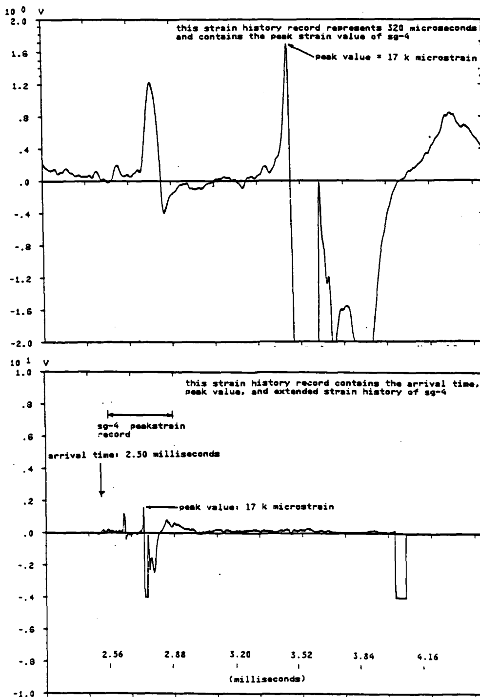
Figure 4.30 Strain Gage NO. 4 Strain History.
