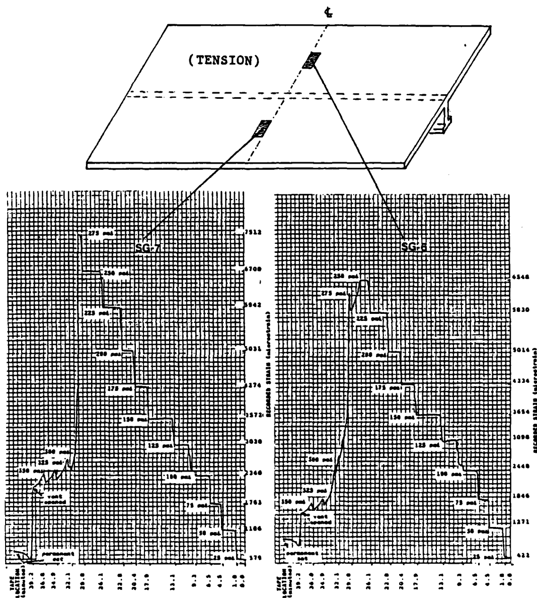
Figure 4.16 Strain History Recorded Across Transverse Centerline of Plate Back.
