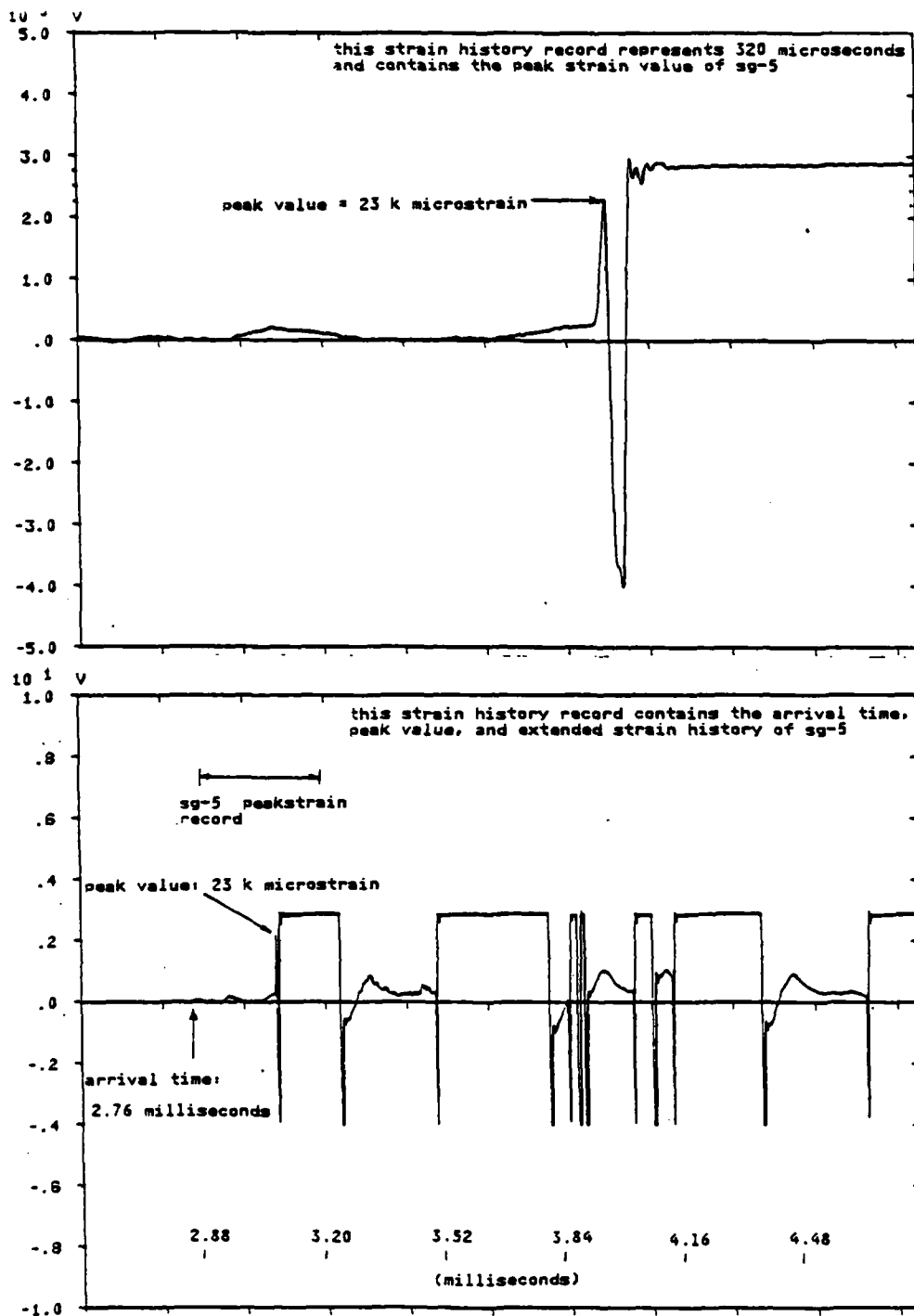
Figure 4.31 Strain Gage NO. 5 Strain History.
