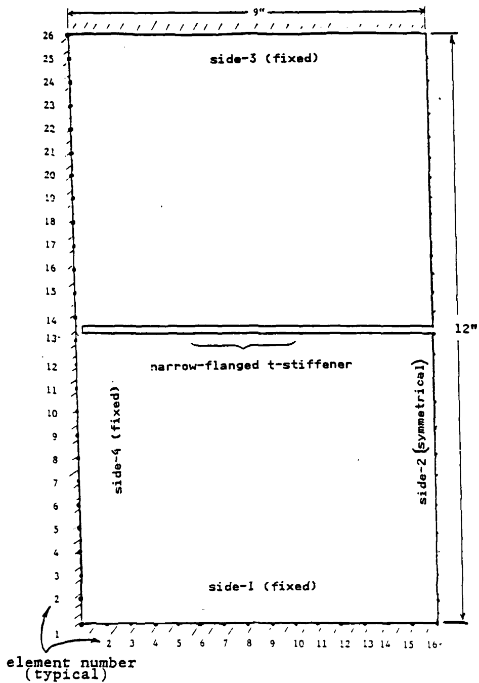
Figure 4.1 Segmentation of Half-plate.
