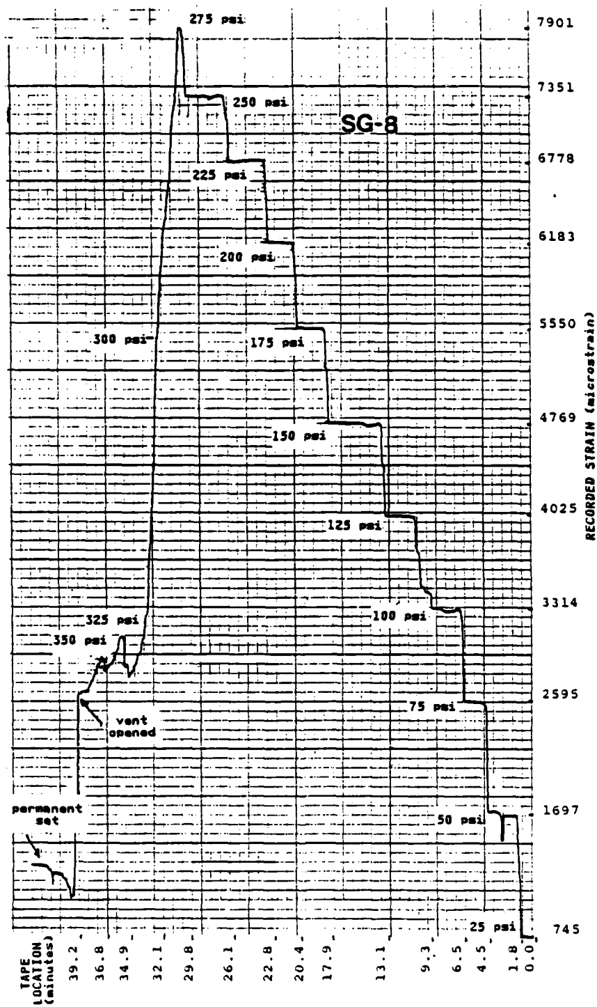
Figure 4.10 Strain Gage NO. 8 Strain History.
