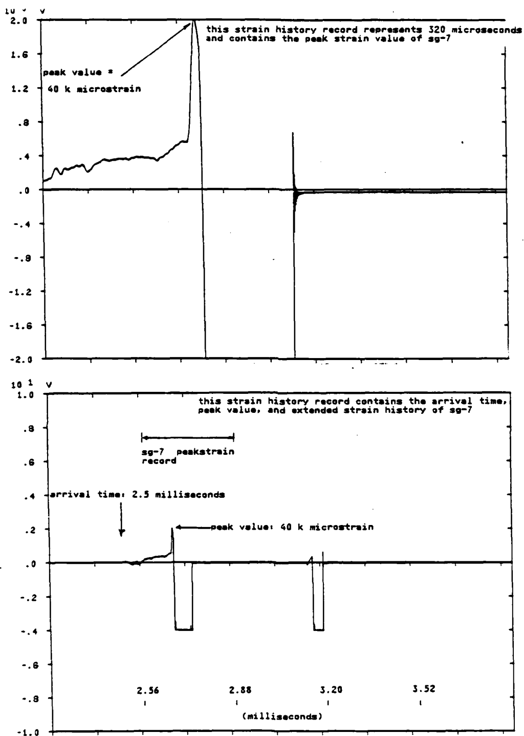
Figure 4.33 Strain Gage NO. 7 Strain History.
