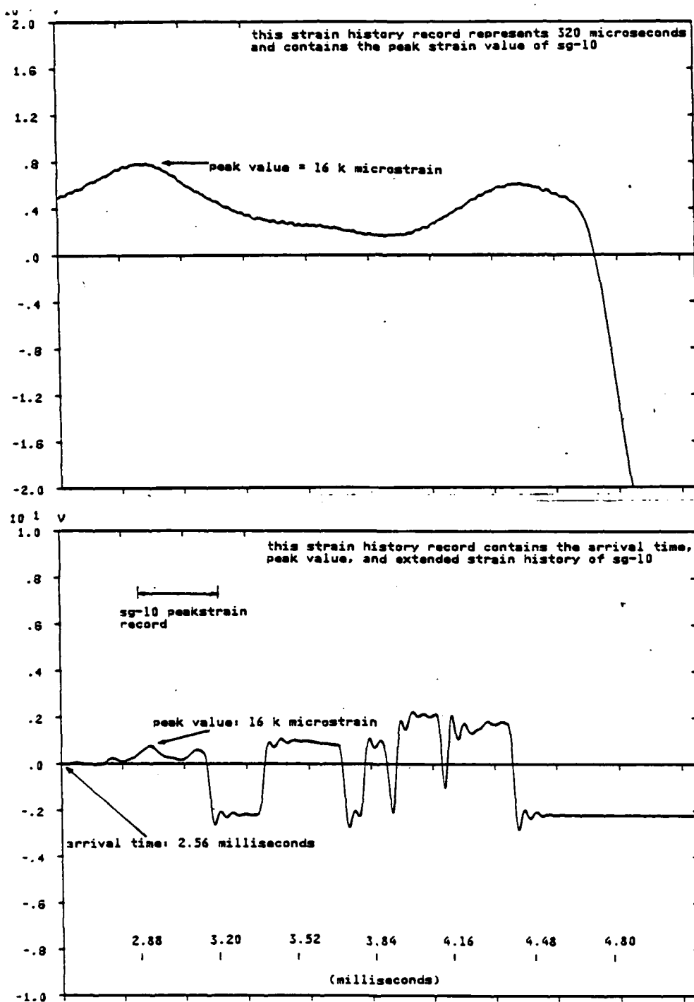
Figure 4.36 Strain Gage NO. 10 Strain History.
