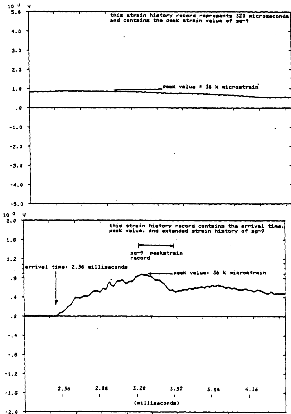
Figure 4.35 Strain Gage NO. 9 Strain History.
