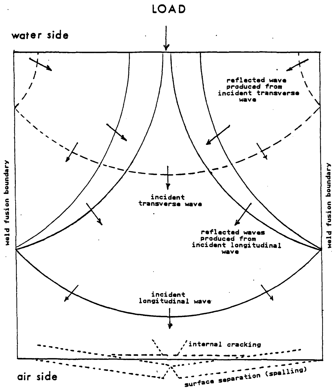
Figure 4.45 (Top) Incident and Reflected Waves in Flat Plate. (Bottom) Depiction of Spalling.
