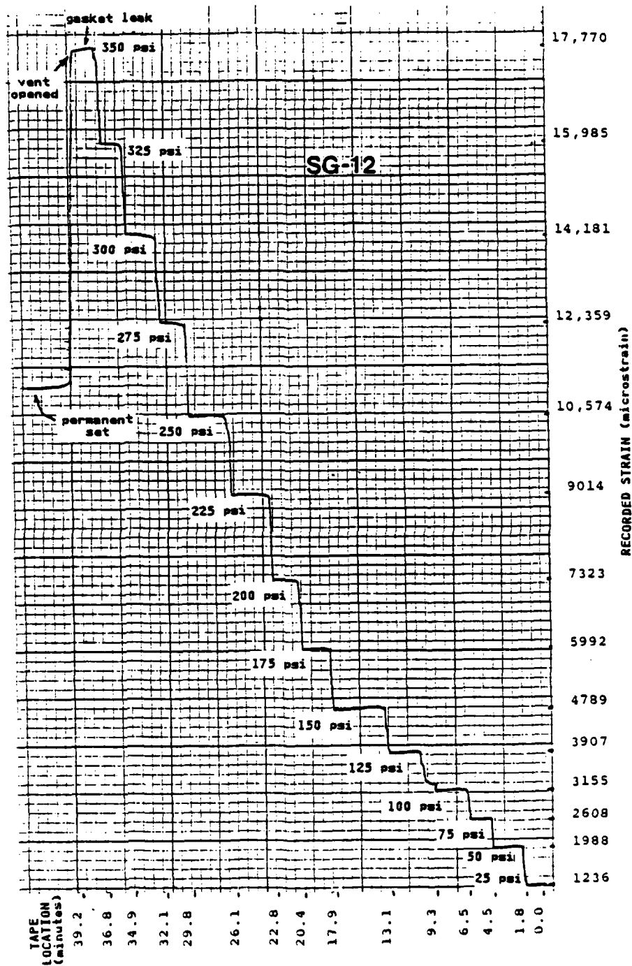
Figure 4.13 Strain Gage NO. 12 Strain History.
