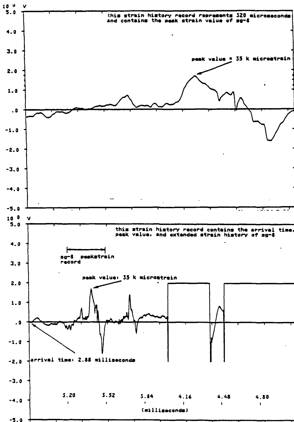
Figure 4.34 Strain Gage NO. 8 Strain History.
