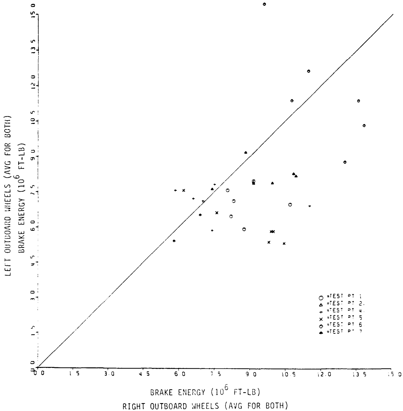
FIGURE 16 - BRAKE ENERGY SCATTER (THERMAL) FHBS TEST PHASE
