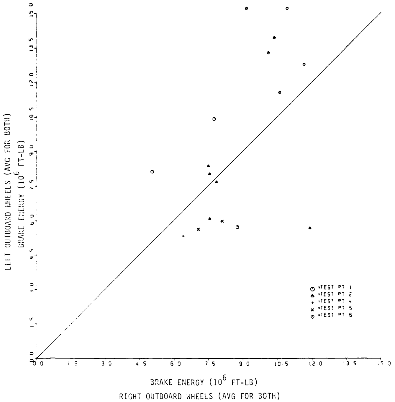
FIGURE 15 - BRAKE ENERGY SCATTER (STRAIN) BASELINE TEST PHASE
