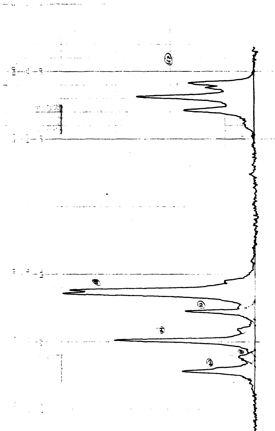
Figure 15. ^1\text{H} NMR Spectrum of DINOL (5)/Dinitroheptanediol (3) Copolyformal (40/60, Table 3, #3), -\text{OCH}_2\text{O}- Region
