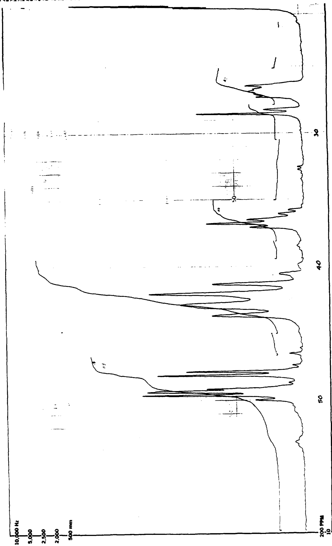
Figure 5. ^1\text{H} NMR Spectrum of Decafluorodiol (2)/Dinitroheptanediol (3) Copolymer (80/20)
