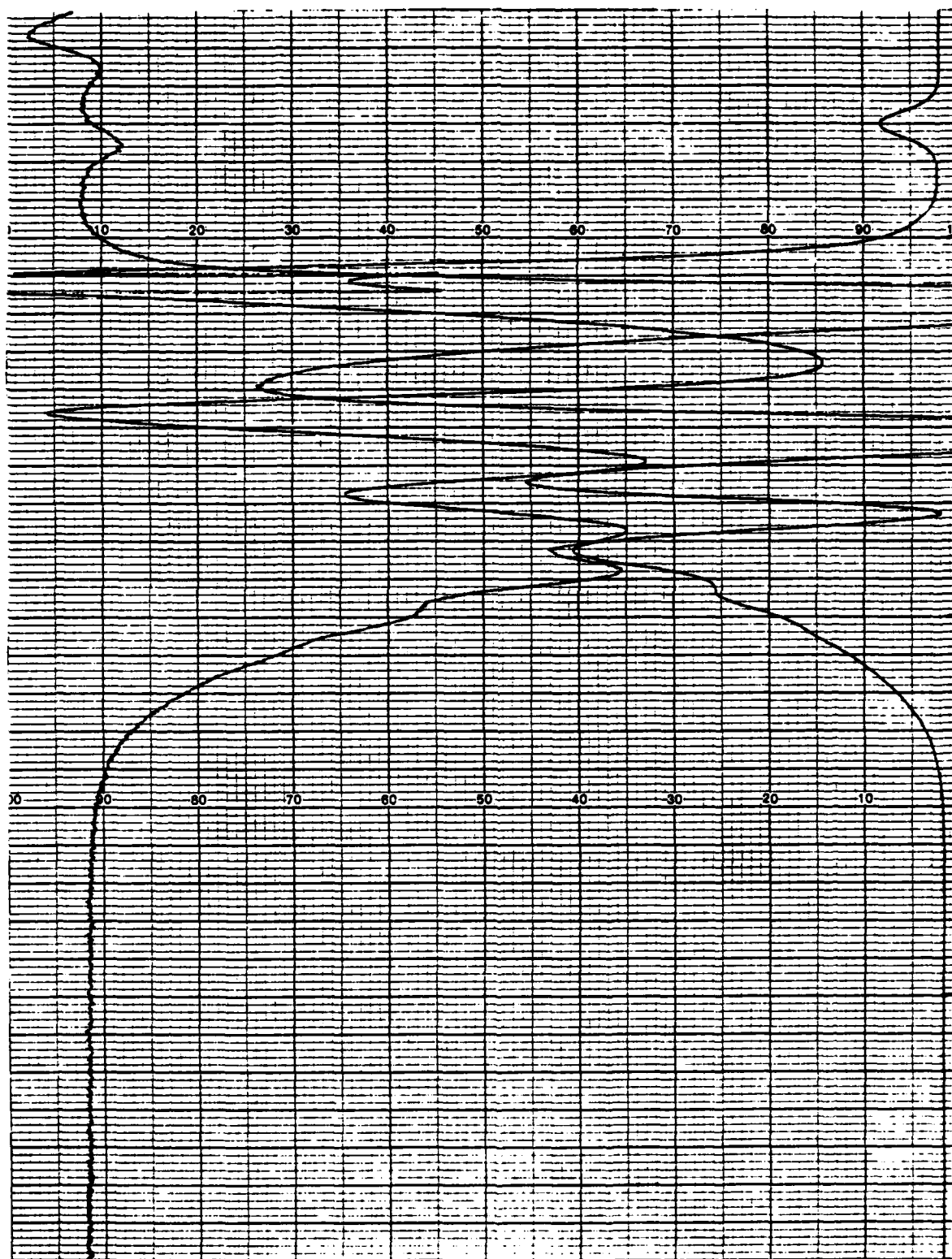
Fig. 8 GP Chromatogram of Attempted Copolymerization of Dioxolane/Dinol (Run #6, Table 2)
