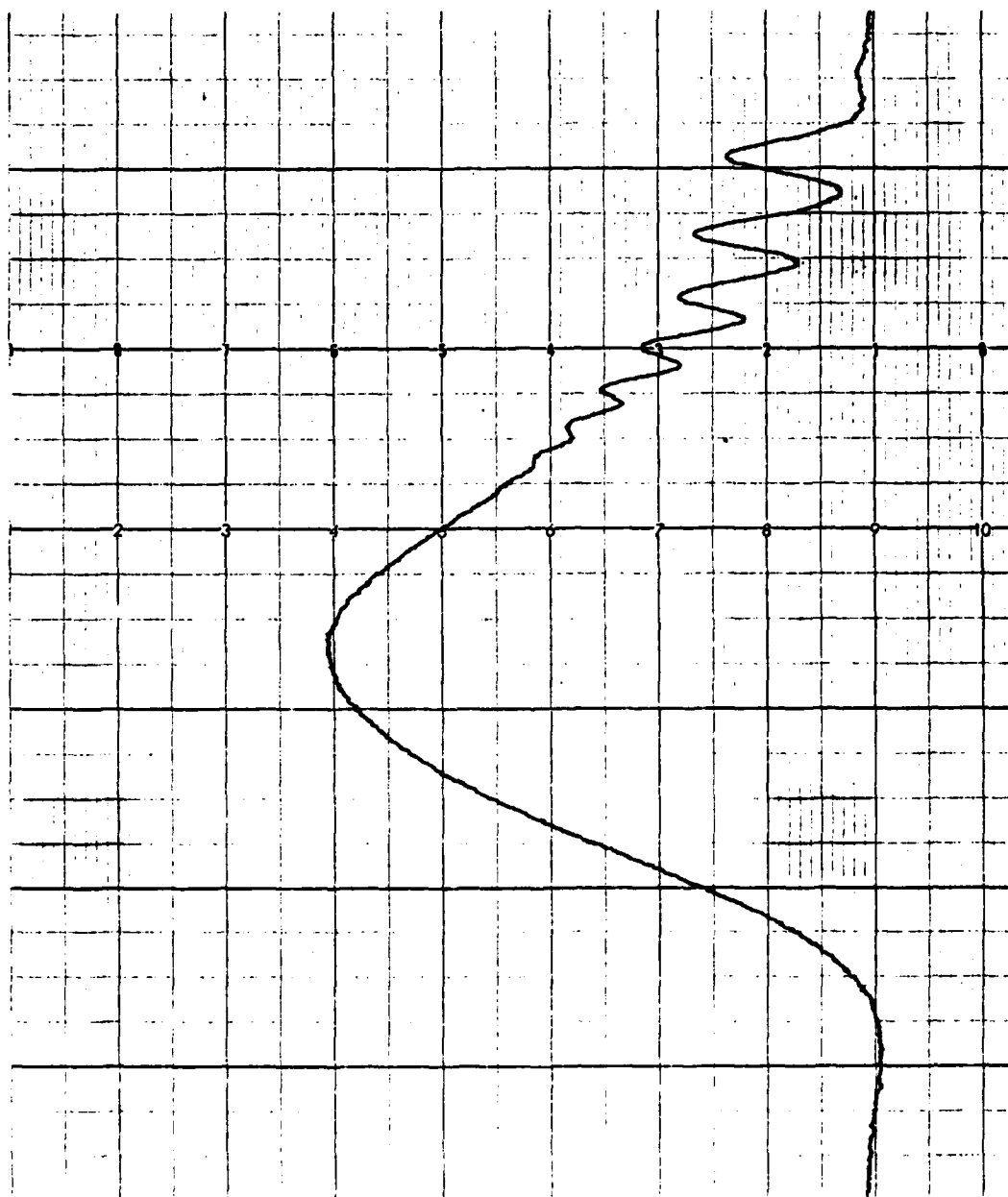
Figure 1. GP Chromatogram of Hexafluoropentanedio1 (1) Polyformal (0.5 1b batch)
