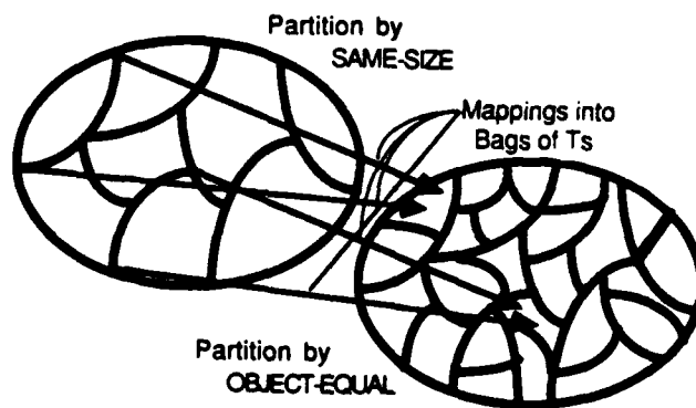
Figure 2 . AM's CANONIZE heuristic found a partition preserving mapping from the domain of SAME-SIZE to the domain of OBJECT-EQUAL. This mapping transformed each element of SAME-SIZE lists into the unique symbol T , producing OBJECT-EQUAL lists.
