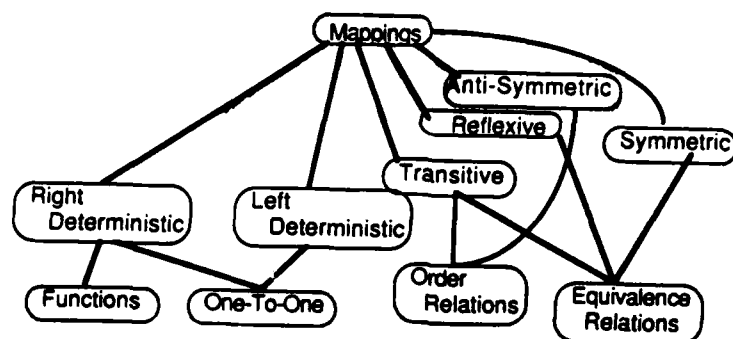
Figure 3. All of Cyrano's concepts and meta-concepts are uniformly represented in a lattice of types.
