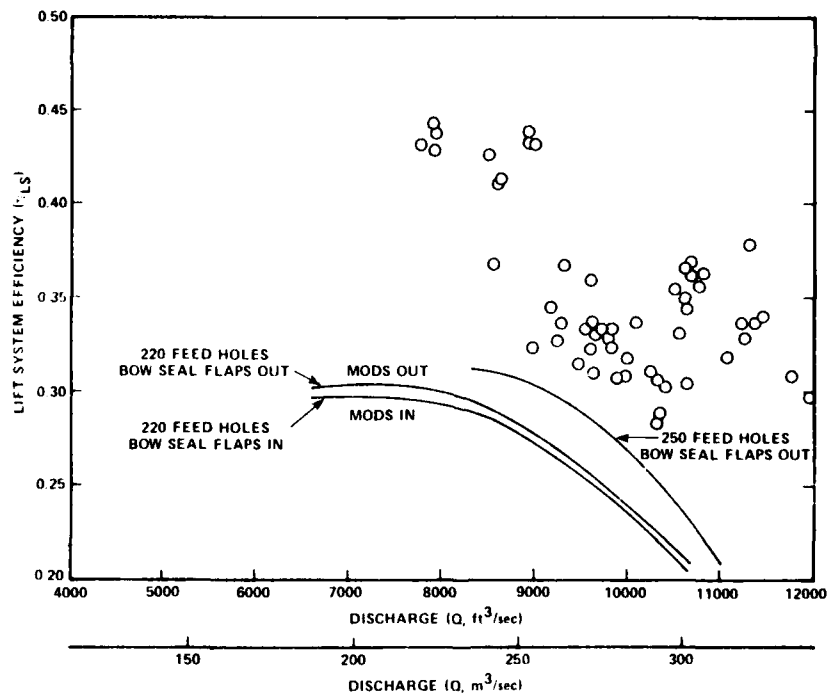
Figure 11 - Variation of Lift System Efficiency with Lift System Flow Rate--Data Correspond to 220 Feed Holes with Bow Seal Flaps Out
