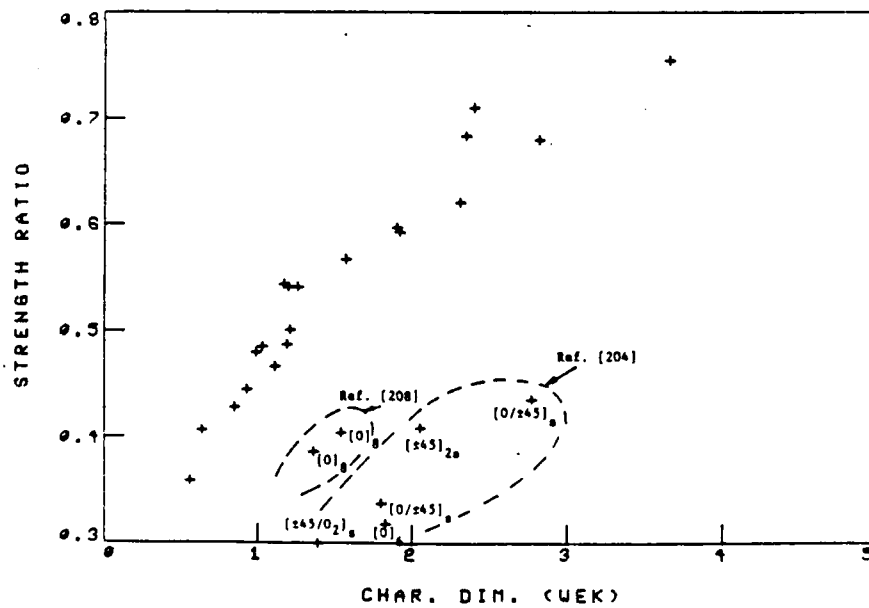
Figure 116. Correlation between notched strength ratio (for 2c/W = 0.3 ) and characteristic dimension, a_c , (WEK-fracture model) for boron/aluminum laminates containing straight cracks.
