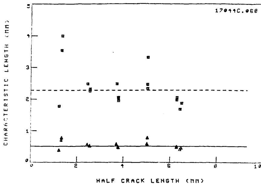
Figure 25. Characteristic dimensions (WN-fracture model) as a function of half crack length for graphite/epoxy [0/90/245]_s laminate (A — "point stress" criterion, d_0 = 0.51 mm; - - - "average stress" criterion, a_0 = 2.26 mm) indicating that both can be considered as material constants.
