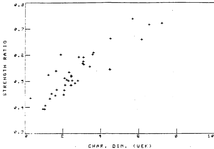
Figure 115. Correlation between notched strength ratio (for 2R/W = 0.25 ) and characteristic dimensions, a_c , (WEK-fracture model) for graphite/epoxy laminates containing circular holes.
