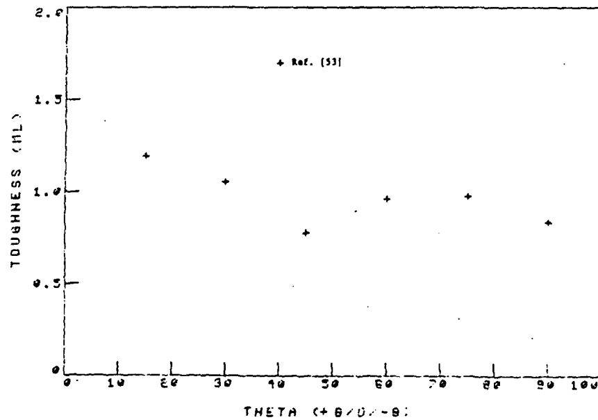
Figure 114. Experimental values of fracture toughness, K_{IC}/c_0 , (ML-fracture model) as a function of angle for graphite/epoxy [+3/0/-3] laminates containing circular holes. Individual data are given in Table 14 and Appendix E.
