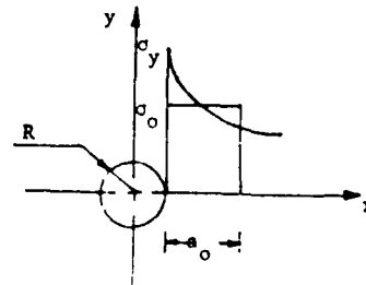
Figure 11. Schematic representation of the "average-stress" criterion [5].
