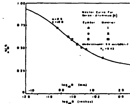
Figure 43. Master curve for boron/aluminum [8].
