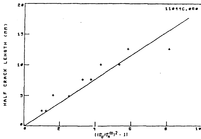
Figure 9. Best fit for a_c (VEK-fracture model) for graphite/epoxy [0/90/\pm 45]_s laminate ( a_c = 1.02 mm).
