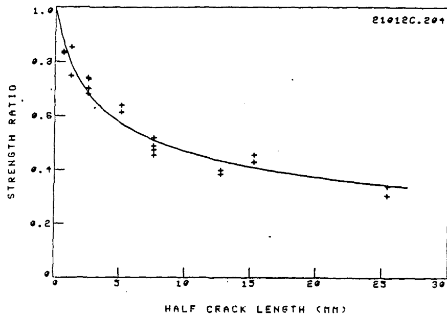
Figure 56. Comparison between experiments and prediction (PWG-fracture model) for boron/aluminum [0/±45] s laminate ( m = 0.23 , K = 0.62 , \bar{a}_{PM} = 26.9 ).
