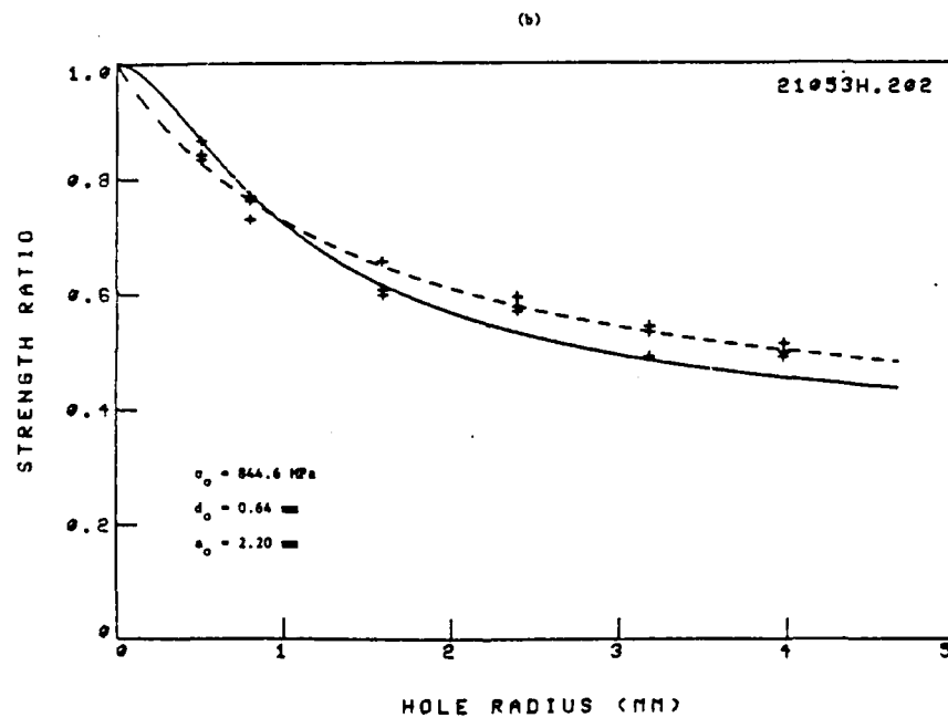
Figure 22. Comparison between experiments and predictions (VN-fracture model) for: a. graphite/epoxy [0/\pm 45/90]_s laminate; b. boron/aluminum [0/\pm 45/0_2]_s laminate (— "point stress" criterion; --- "average stress" criterion).
