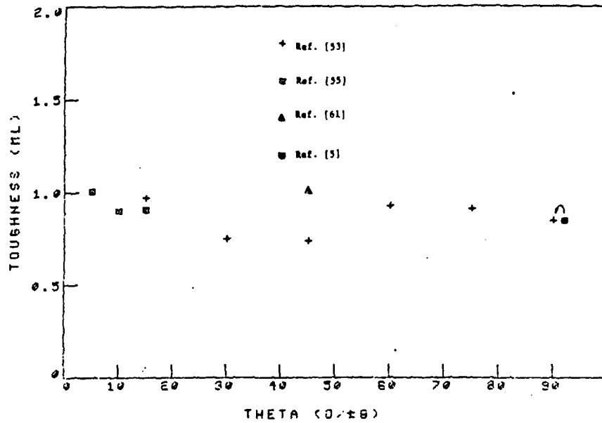
Figure 113. Experimental values of fracture toughness, K_{IC}/c_0 , (ML-fracture model) as a function of angle for graphite/epoxy [0/\pm 3] laminates containing circular holes. Individual data are given in Table 14 and Appendix E.
