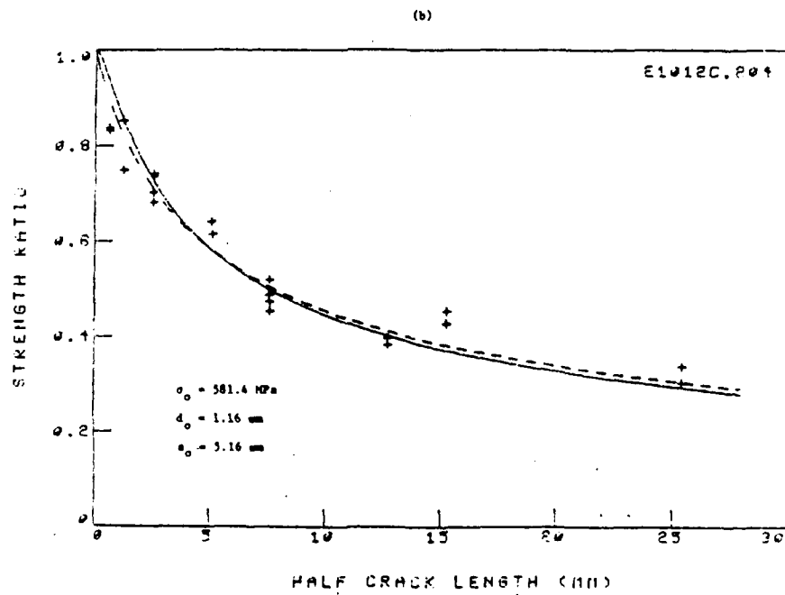
Figure 23. Comparison between experiments and predictions (UN-fracture model) for: a. graphite/epoxy [0/90/45]_s laminate; b. boron/aluminum [0/45]_s laminate. (— "point stress" criterion; --- "average stress" criterion).
