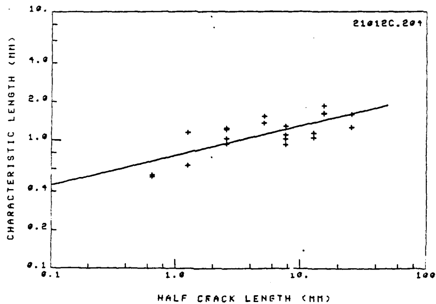
Figure 57. Characteristic dimension (PWG-fracture model) as a function of half crack length for boron/aluminum [0/±45] s laminate ( m = 0.23 , K = 0.62 , \bar{a}_{PM} = 26.9 ).
