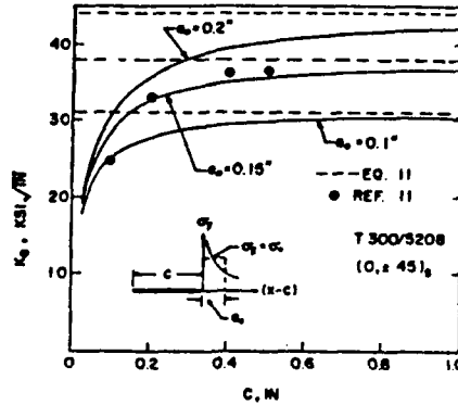
Figure 19. Critical stress intensity factor as a function of crack length for graphite/epoxy laminates, point stress criterion [4]. Data taken from [28].
