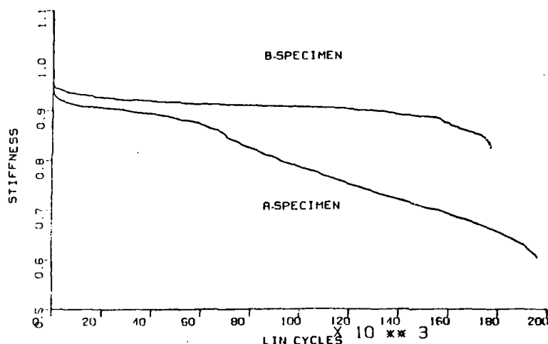
Figure 6. Stiffness Degradation Versus Linear Cycles
