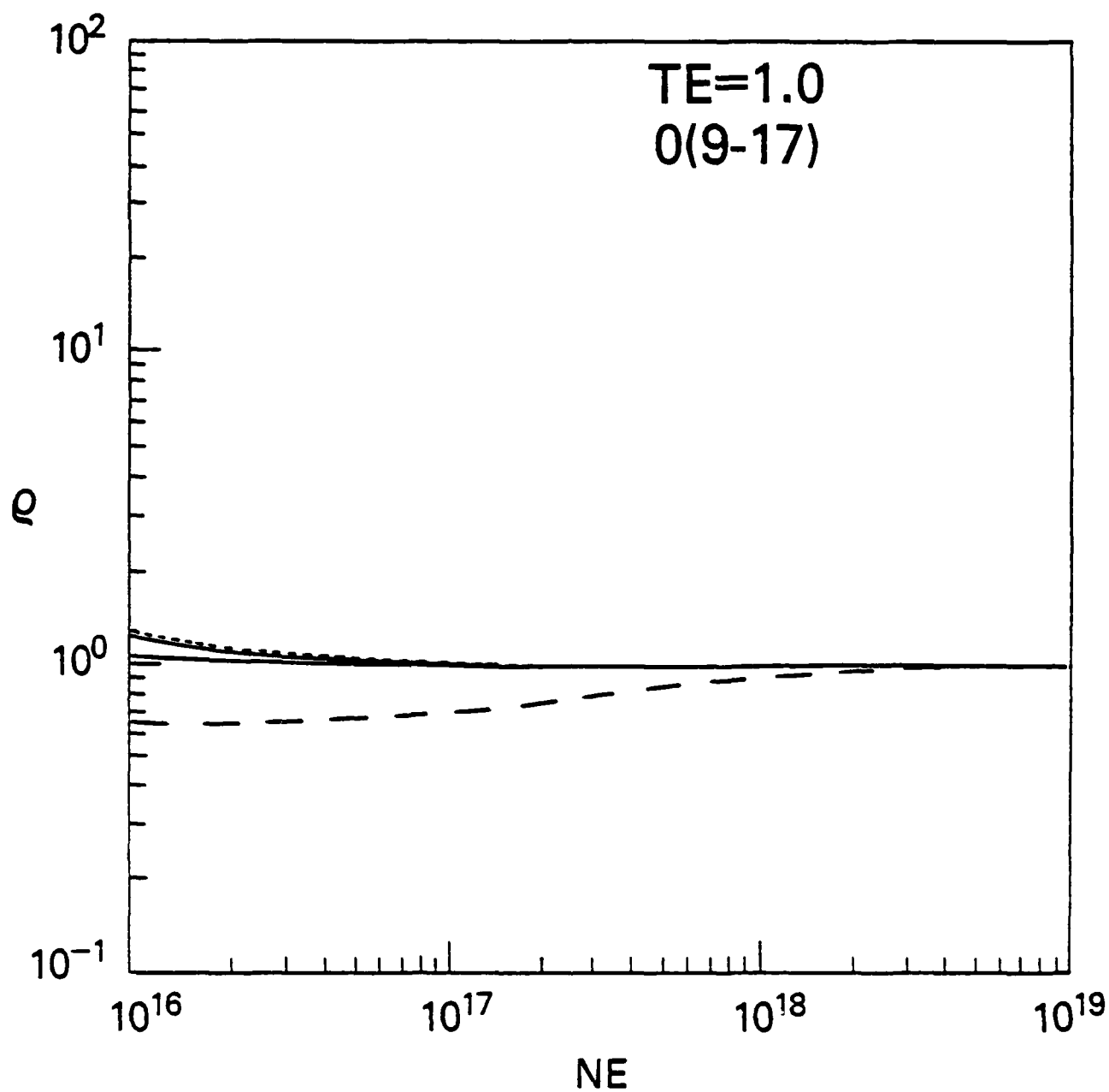
Fig. 2. Saha decrements, T_e=1.0 eV. The initial order from top to bottom is \rho(10) , \rho(12-16) , \rho(9,11) and \rho(17) .
