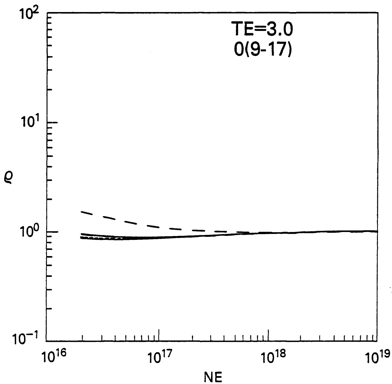
Fig. 18. Saha decrements, T_e=3.0 eV; as in Fig. 14.
