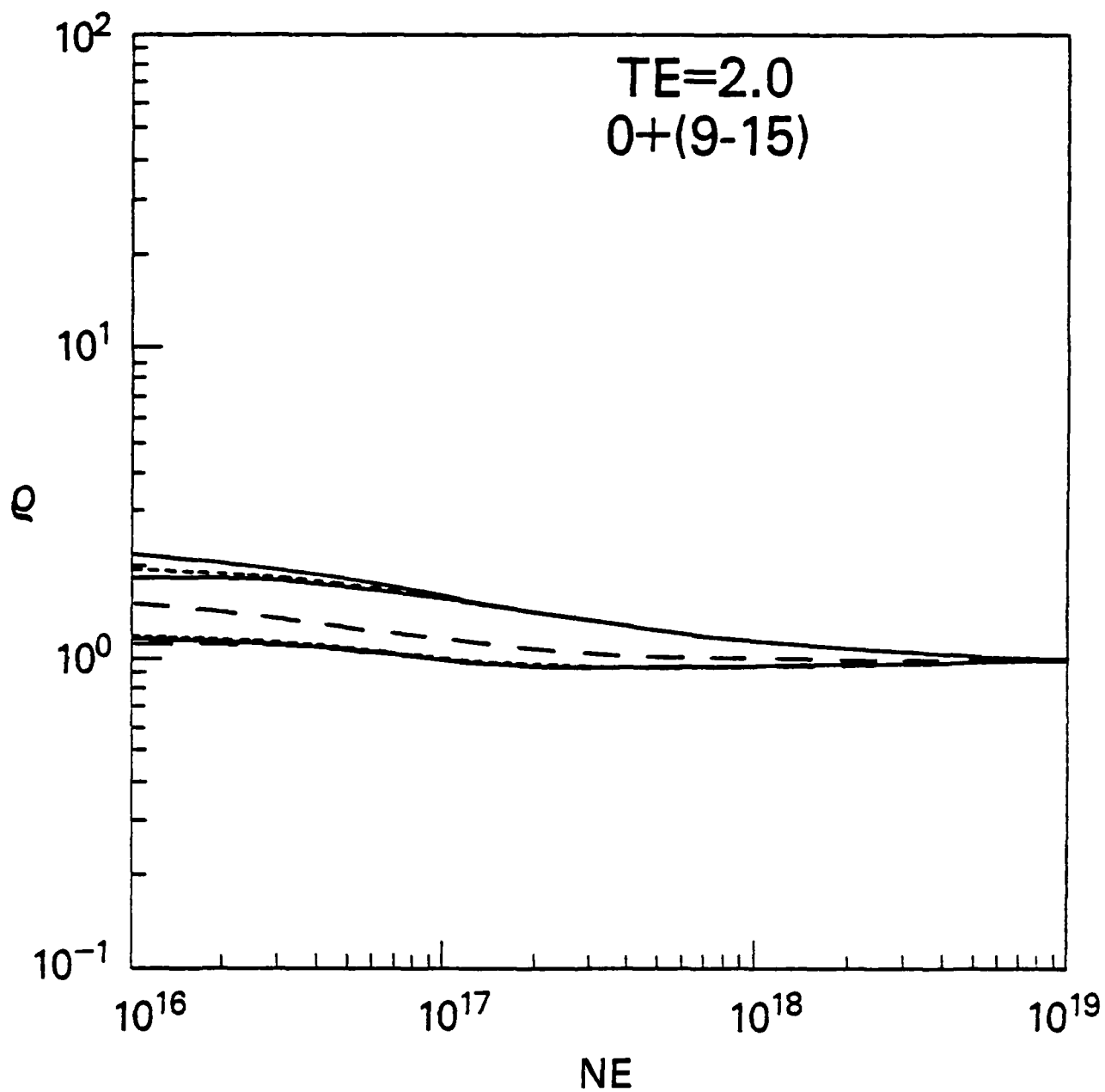
Fig. 12. Saha decrements, T_e=2.0 eV; as in Fig. 8.
