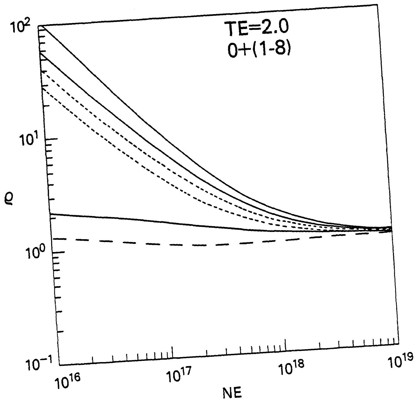
Fig. 11. Saha decrements, T_e=2.0 eV; as in Fig. 7.
