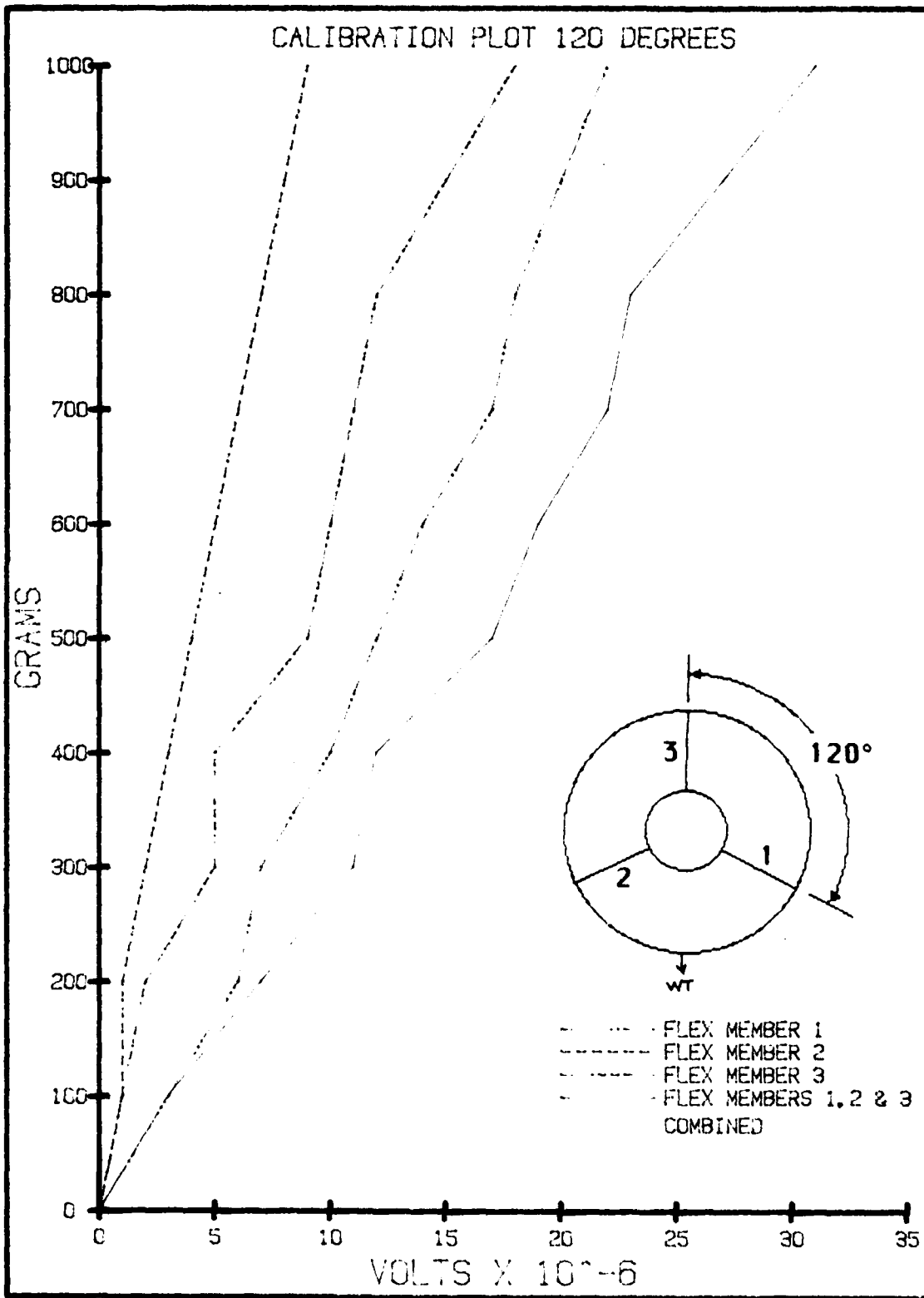
Figure 41. Calibration Plot 120 Degrees Using an Hp 3497
