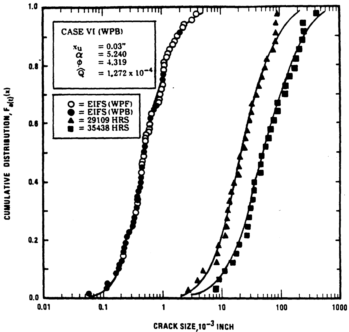
Figure 77: Correlation Between Predictions and Test Results for the Cumulative Distribution of Crack Size at 29109 and 35438 Flight Hours for WPB Data Set (Case VI: Pooled EIFSs for WPF + WPB; Normalized Q Value)
