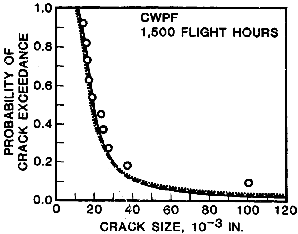
Figure 33: Correlation Between Lognormal Random Variable Model and Test Results for the Probability of Crack Exceedance at 1,500 Flight Hours for CWPF Fastener Holes.
