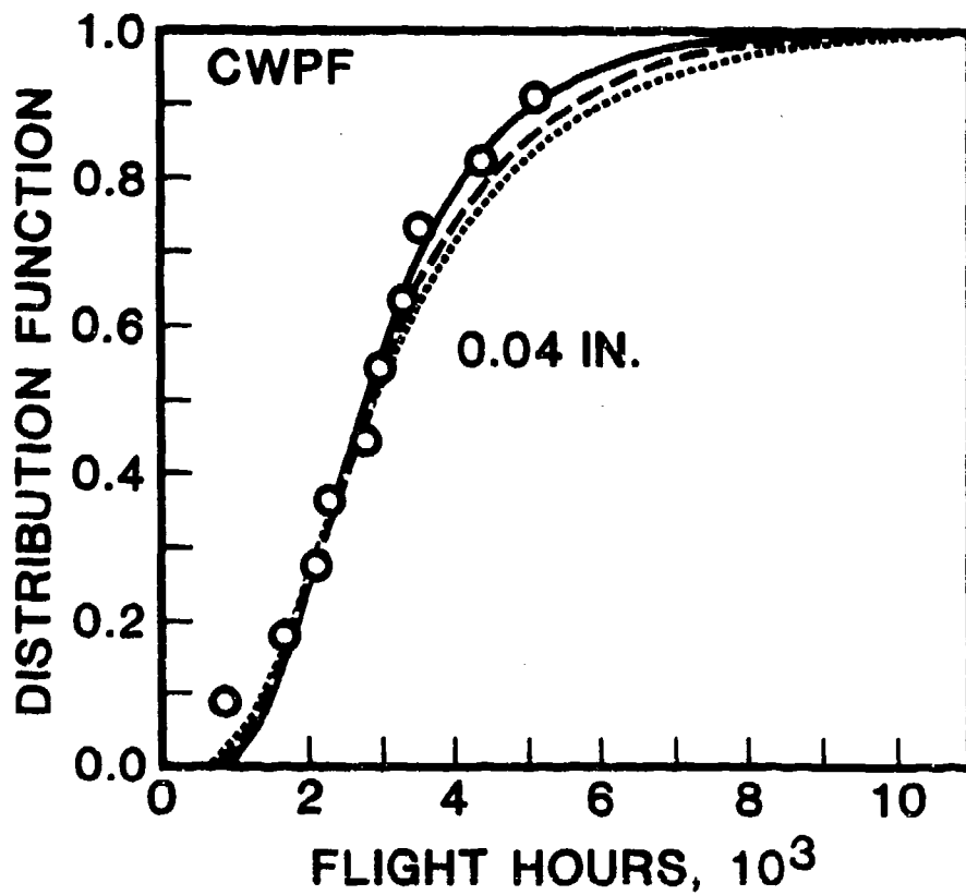
Figure 28(a): Correlation Between Lognormal Random Variable Model and Test Results for the Distribution of Time to Reach 0.04 Inch Crack for CWPF Fastener Holes.
