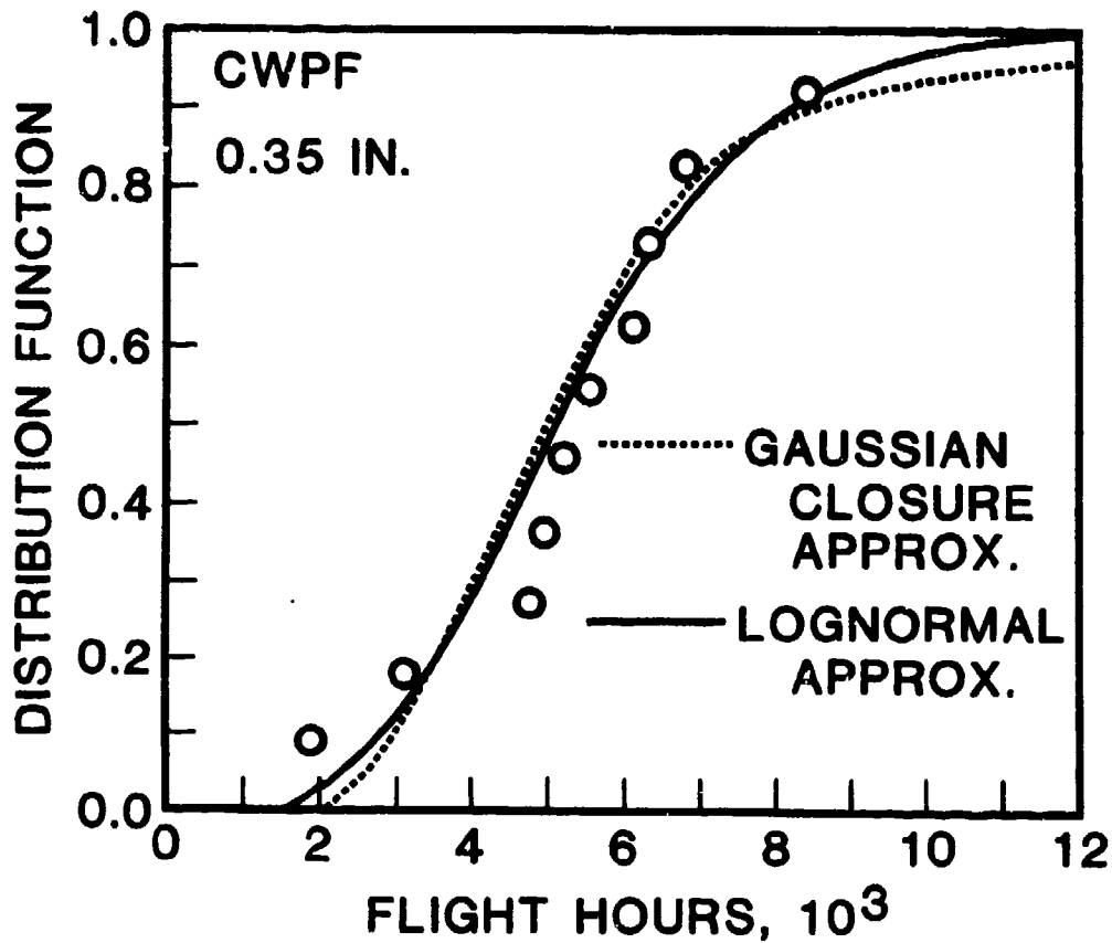
Figure 53(b-3): Correlation Between Second Moment Approximations and Experimental Results for the Distribution of Time to Reach Crack Size of 0.35 Inch for CWPF Fastener Holes; Gaussian Closure and Lognormal Approximations.
