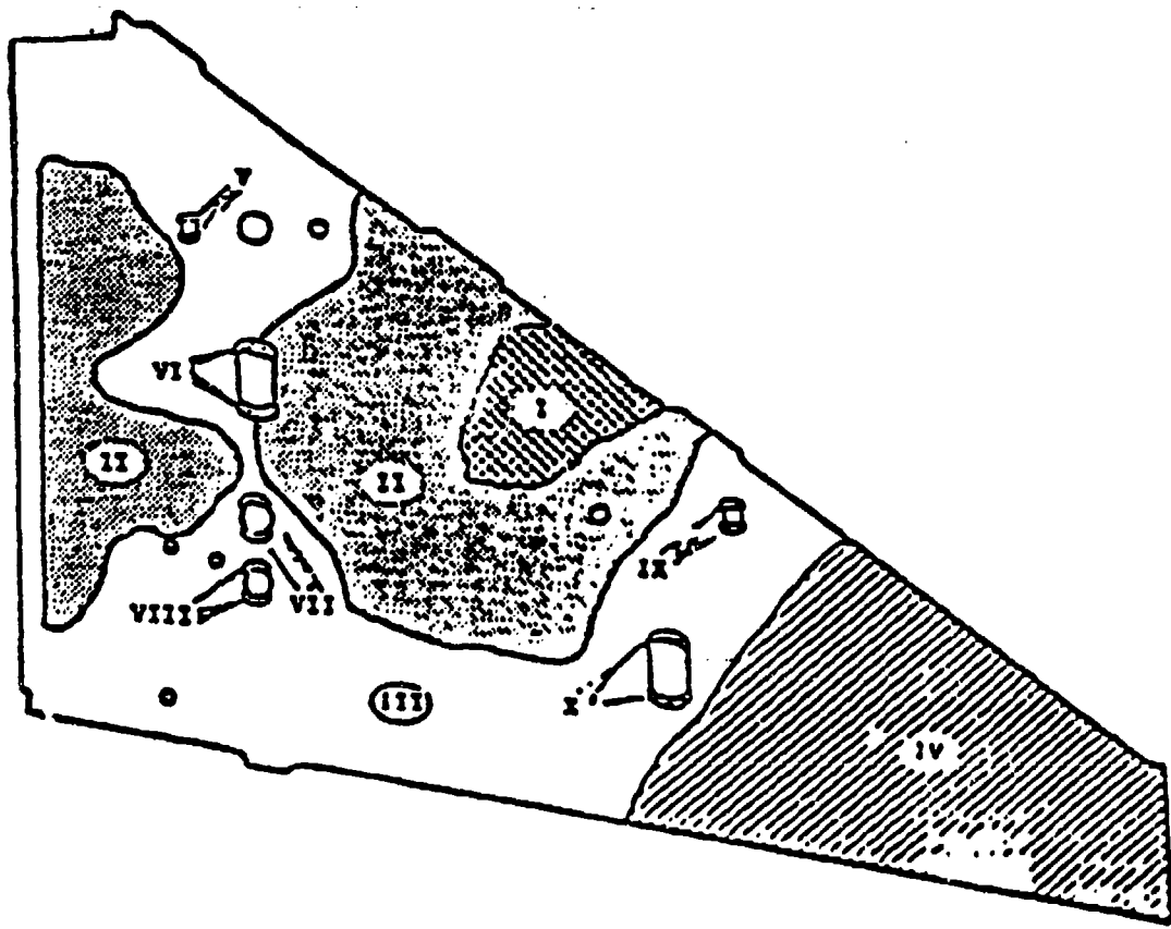
Figure 85: Stress Zones for F-16 Lower Wing Skin
