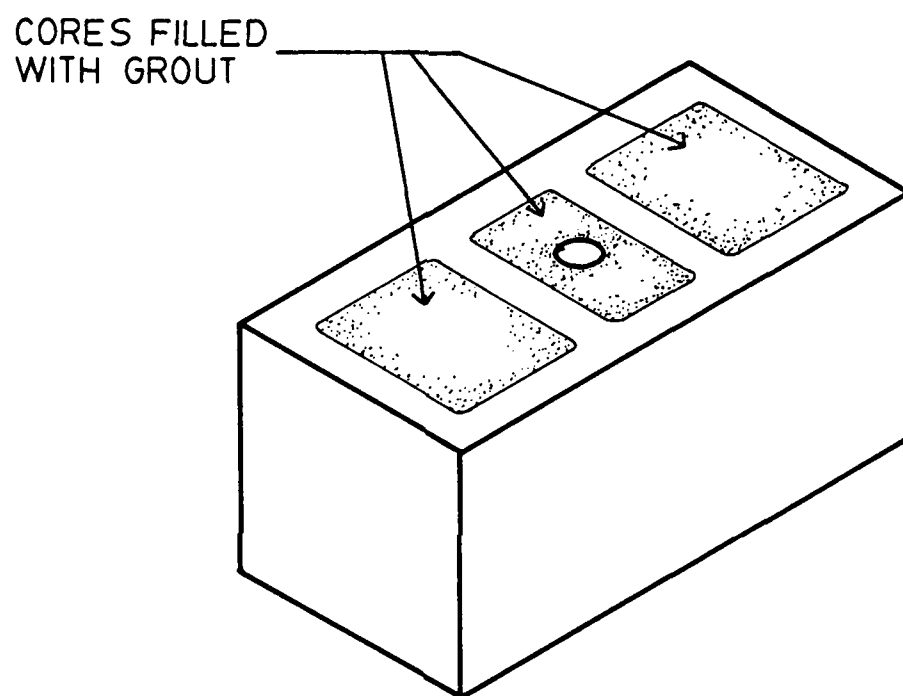
Figure 7.3. Bearing Block.
