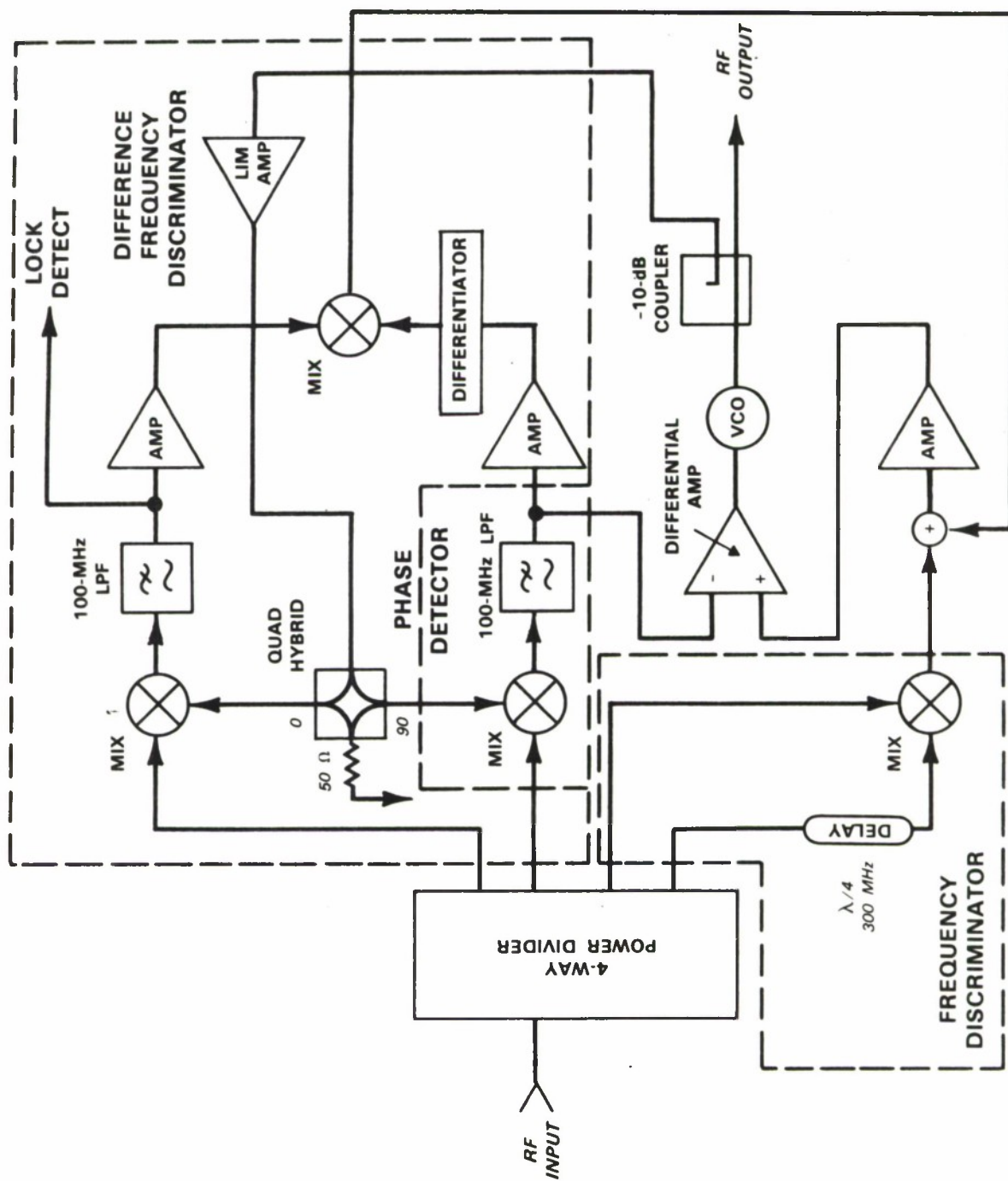
Figure 5-9. Phase-locked loop.
