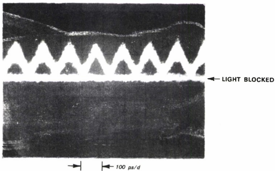
Figure 1-8. Response of back-illuminated n-InGaAs device to 10-GHz output of intracavity-loss modulator laser.
