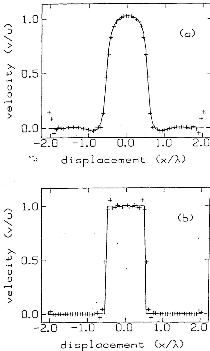
Fig. 4.3 (a) Real part of the reconstructed z-component of the particle velocity field at 0.06 \lambda from the source starting from the pressure 0.13 \lambda from the source. (b) Real part of the z-component of the particle velocity as reconstructed in the source plane from the input source plane pressure. The reciprocal of g_N^{(5)}(z) with filtering was used in both, and in both, the solid line is theory.
