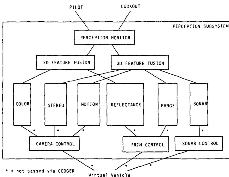
Figure 3-6: The PERCEPTION Subsystem Plan
