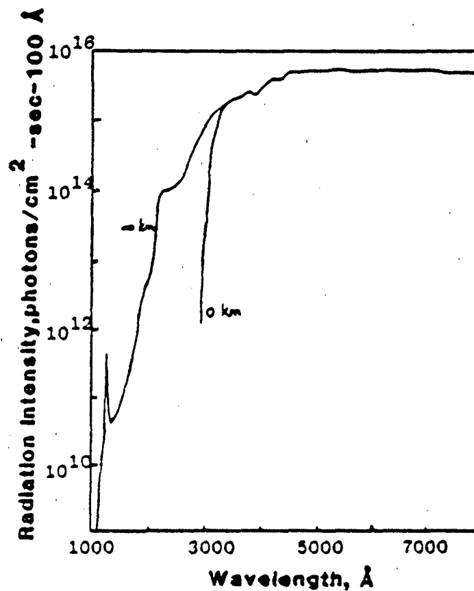
Fig. 2 — Relative intensity of solar radiation as a function of wavelength, at earth's surface (0km) and upper atmosphere (∞km)
