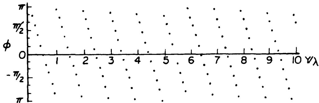
Fig. 2-4. Current distribution for a transmission line radiator (2d=0.1\lambda, Z_T = 160 \Omega)
