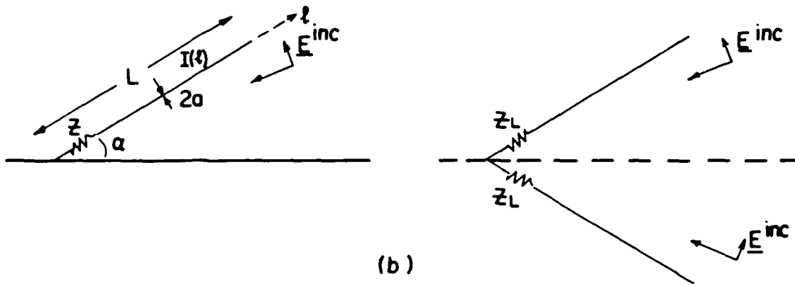
Fig. 2-16. Geometry for a non-uniform transmission line. (a) radiator (b) scatterer
