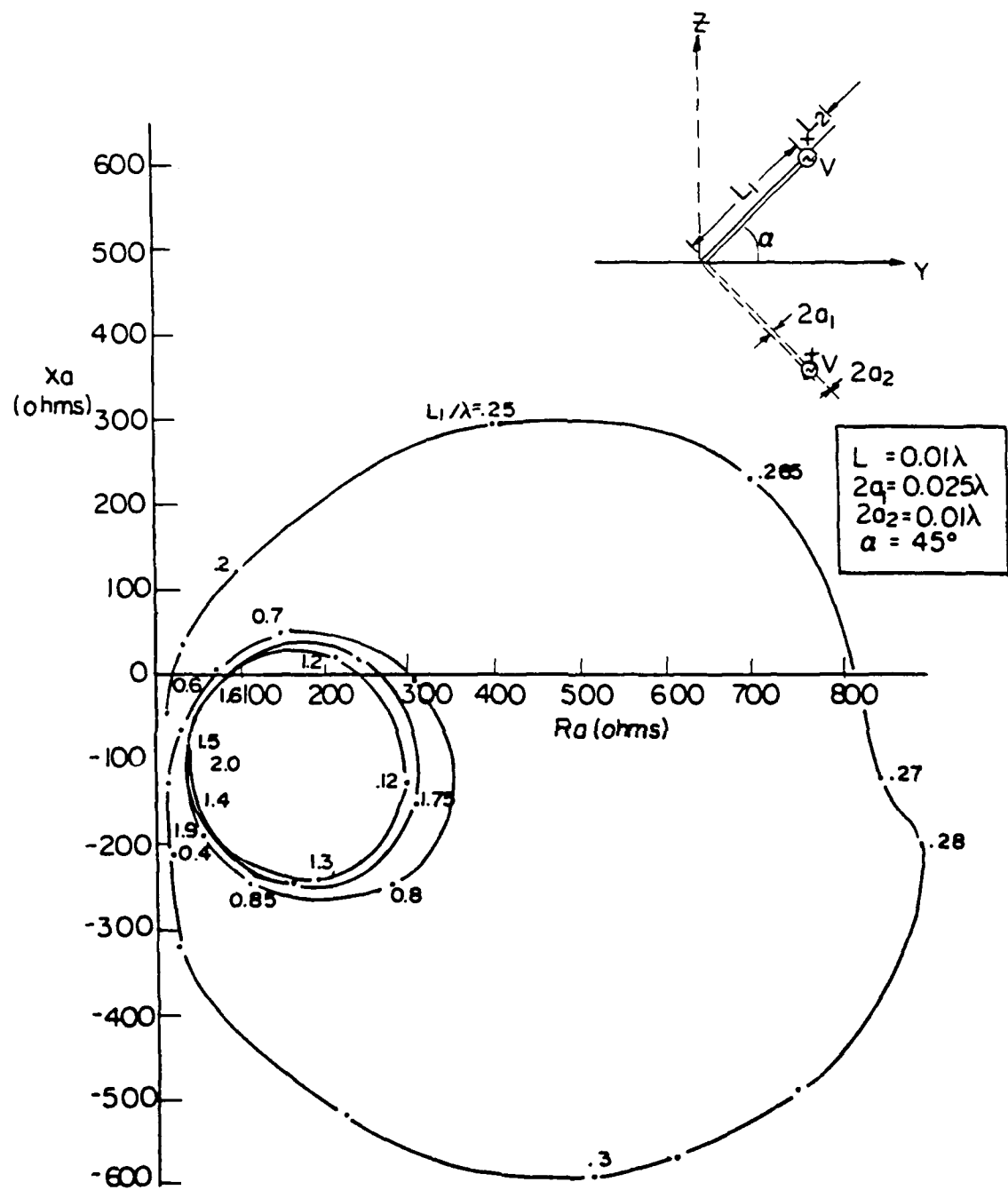
Fig. 4-12. Impedance of a coaxial VEE transmission line ( L_2 = 0.01\lambda ).
