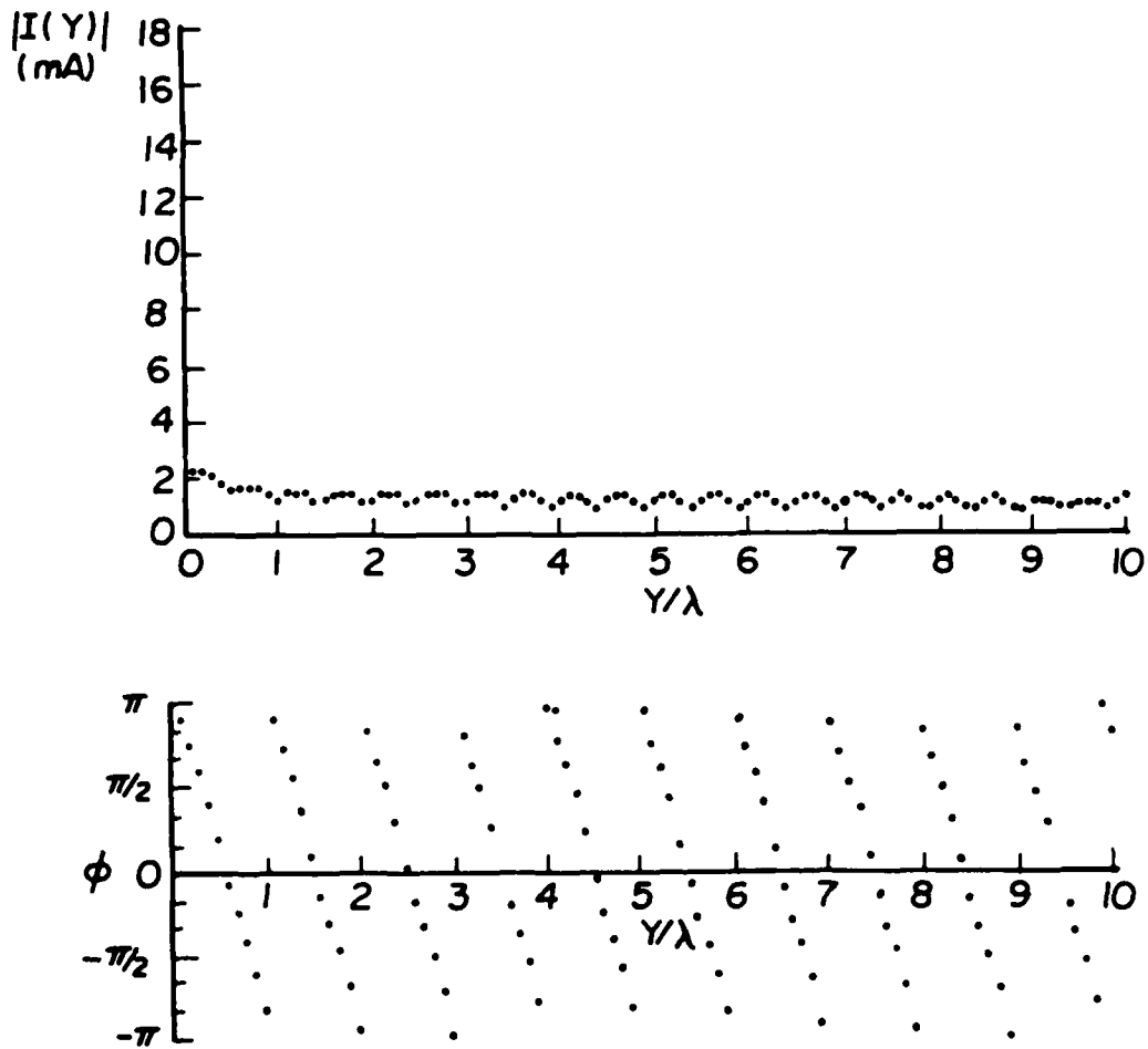
Fig.2-10. Current distribution for a transmission line radiator ( 2d=1.0\lambda, Z_t = 317.9\Omega )
