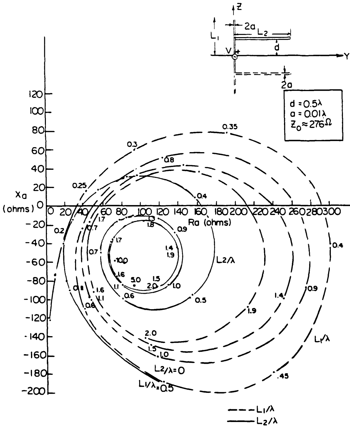
Fig. 4-2. Impedance of the dipole/transmission line ( d = 0.5\lambda )
