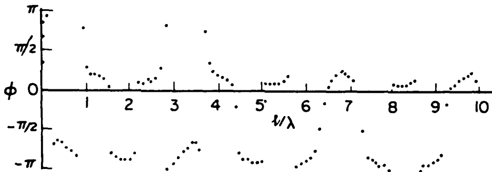
Fig. 2-20. Current distribution for VEE scatterer ( \theta_0 = \phi_0 = 0^\circ )
