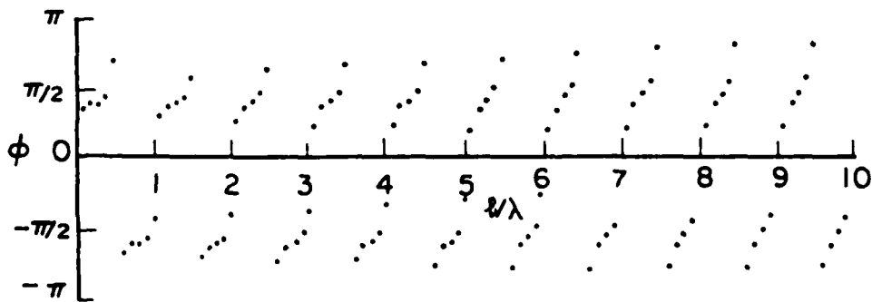
Fig. 2-25. Current distribution for a curved transmission line ( d = 0.1\lambda )
