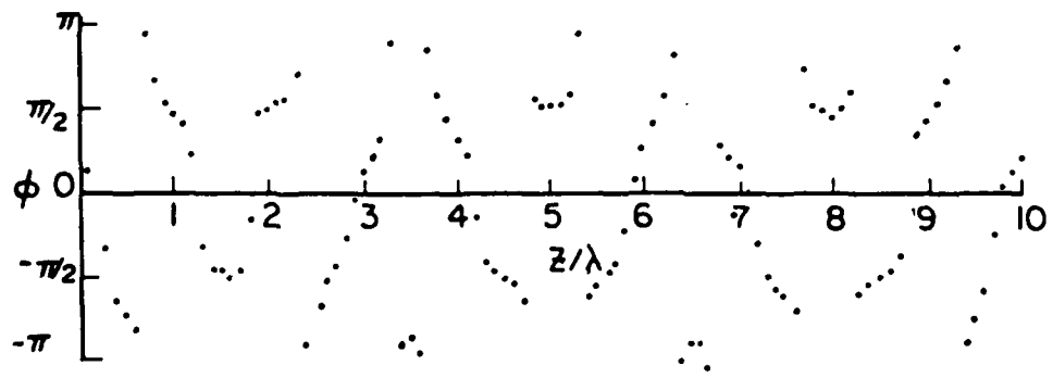
Fig. 2-23. Current distribution for a dipole scatterer ( \theta_0 = 45^\circ , \phi_0 = 270^\circ )
