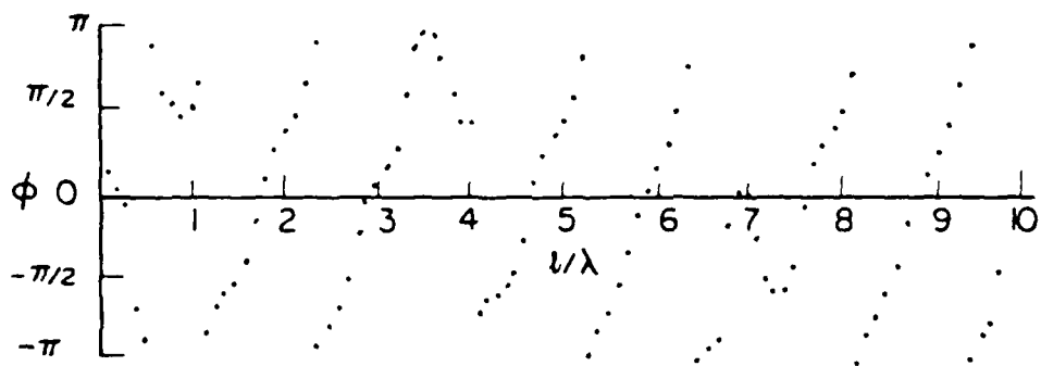
Fig. 2-18. Current distribution for a VEE scatterer ( \theta_0 = \phi_0 = 90^\circ ).
