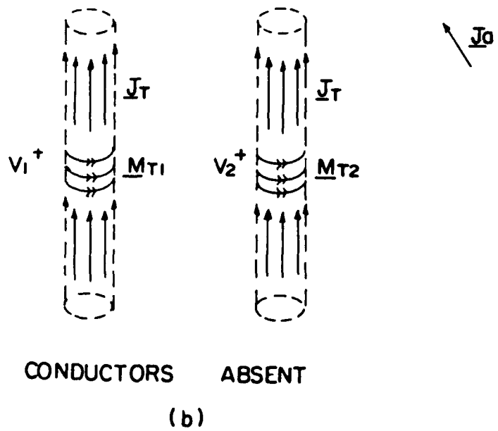
Fig. 3-4. The two-port receiving antenna with voltage sources (a) conductors present (b) conductors absent
