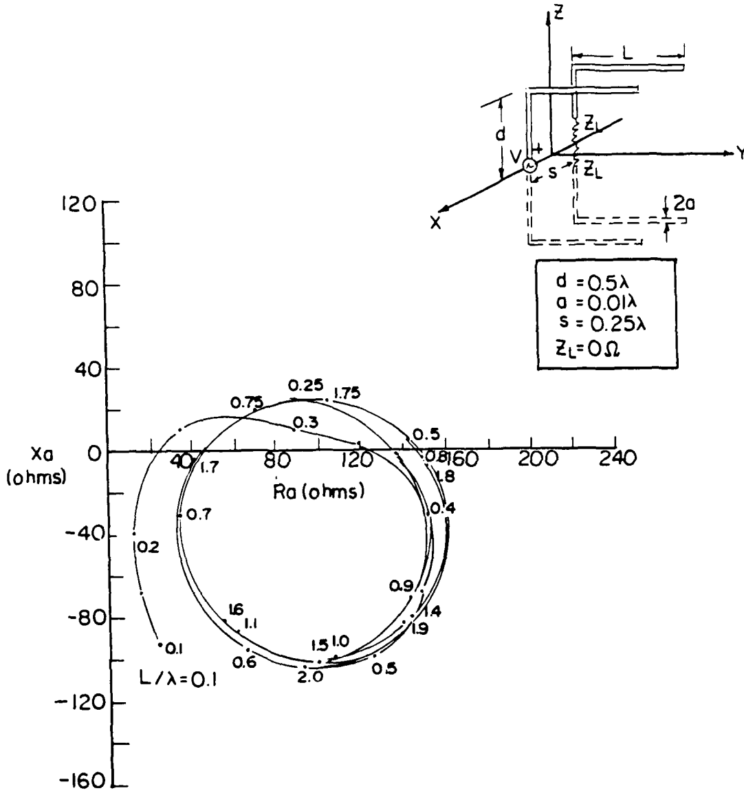
Fig. 4-4. Impedance of a two-conductor transmission line ( S = 0.01 , Z_L = 50\Omega ).
