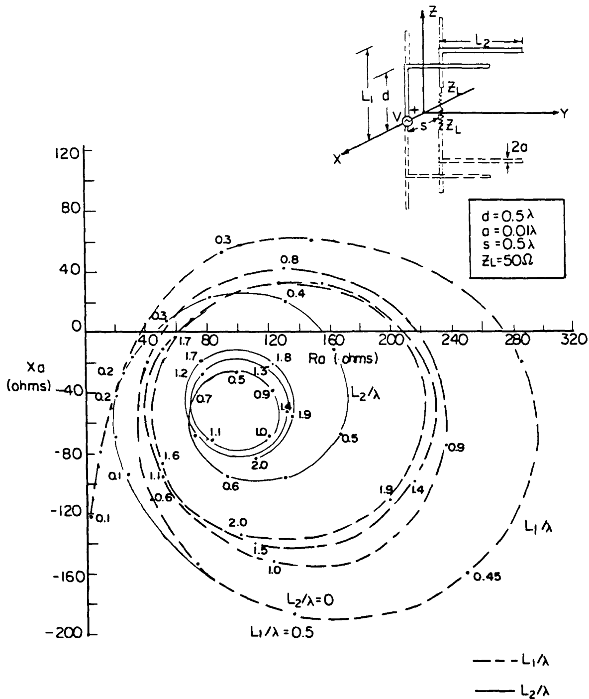
Fig. 4-9. Impedance of a two-conductor transmission line ( S = 0.5\lambda , Z_L = 50\Omega ).
