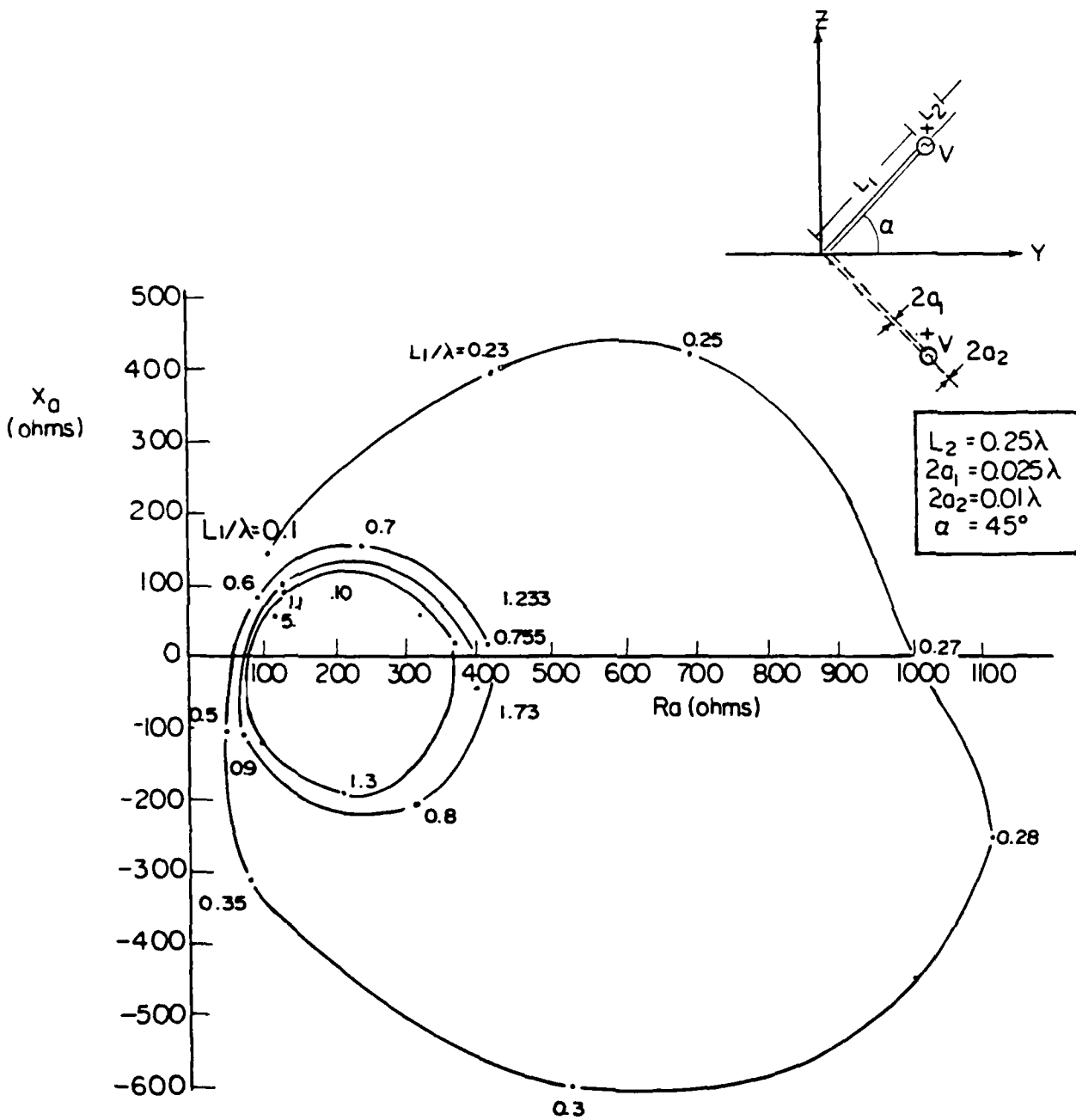
Fig. 4-13. Impedance of a coaxial VEE transmission line ( L_2 = 0.25\lambda ).
