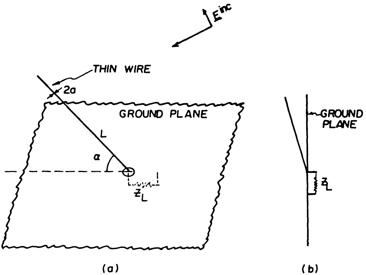
Fig. 1-2. Coupling to a non-uniform (vee) transmission line.
