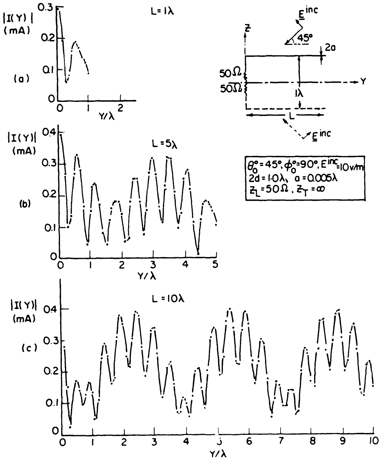
Fig. 2-15. Current distribution for a transmission line scatterer. (a) L = 1 . (b) L = 5 . (c) L = 10 .
