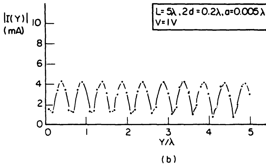
Fig. 2-3. Current distributions for an open-circuited uniform transmission line radiator (a) 2d = 0.1\lambda (b) 2d = 0.2\lambda
