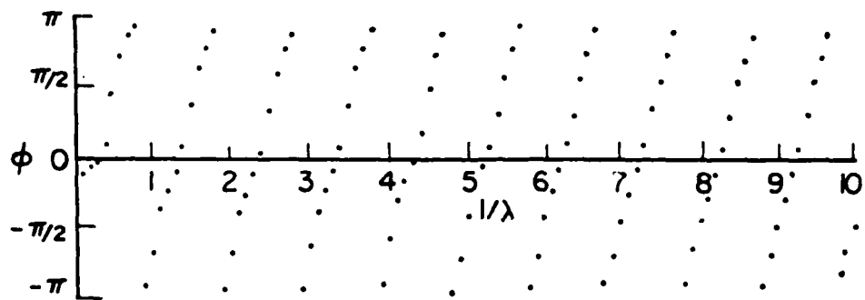
Fig. 2-26. Current distribution for a curved transmission line ( d = 0.5\lambda )
