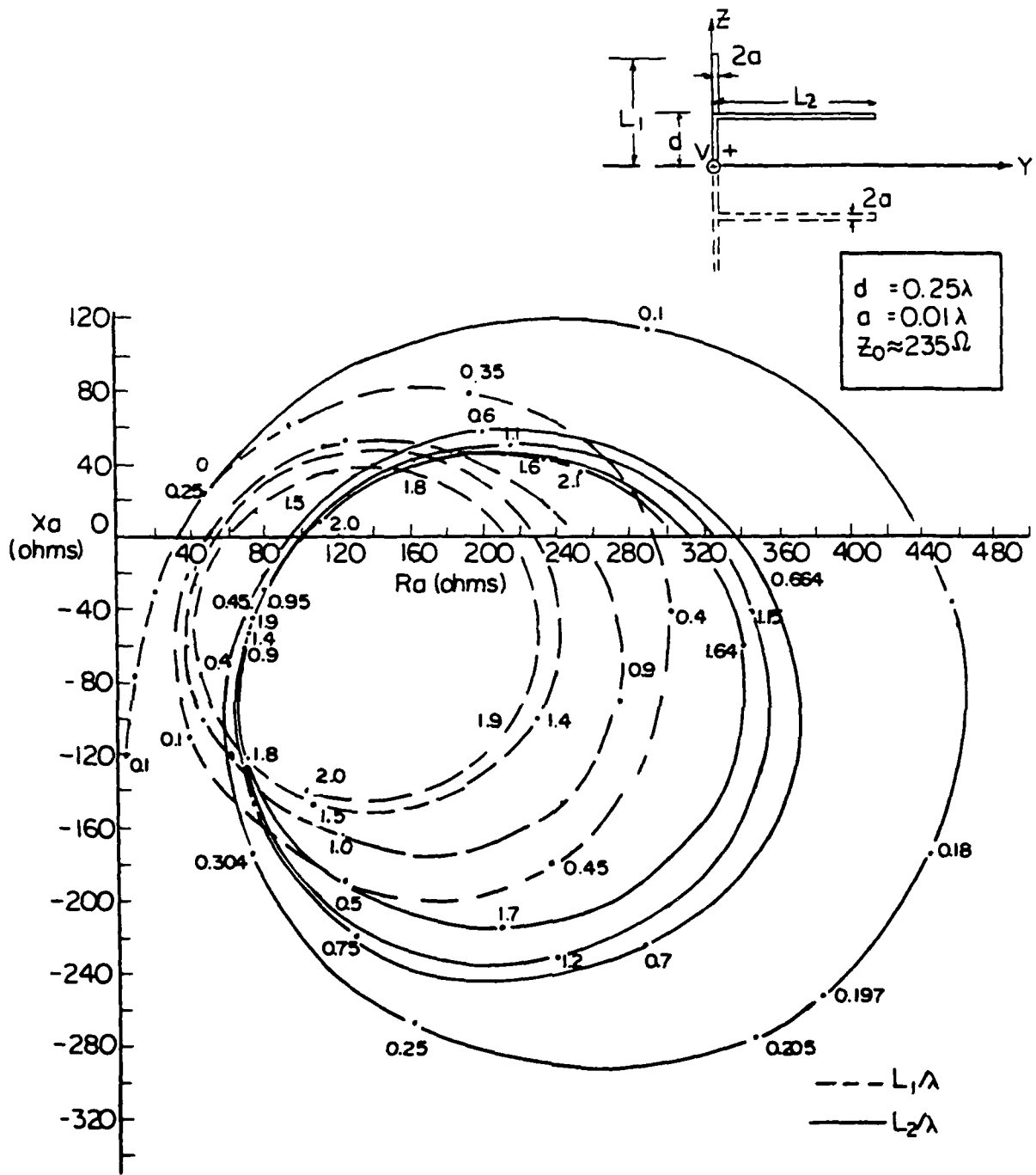
Fig. 4-1. Impedance of the dipole/transmission line ( d = 0.25\lambda )
