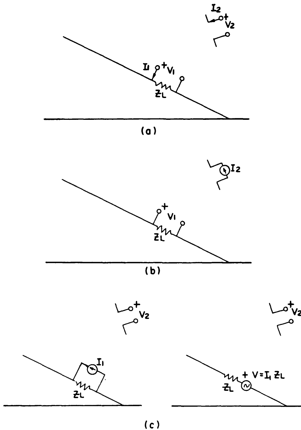
Fig. 2-1. Reciprocity for field-to-wire coupling (a) Basic problem #1 (b) Scattering problem #1 (c) Radiation problem #1
