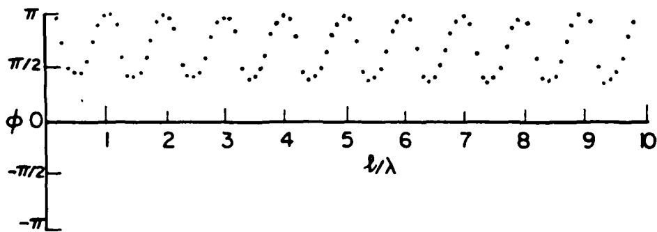
Fig. 2-21. Current distribution for a VEE scatterer ( \theta_0 = 45^\circ , \phi_0 = 270^\circ )
