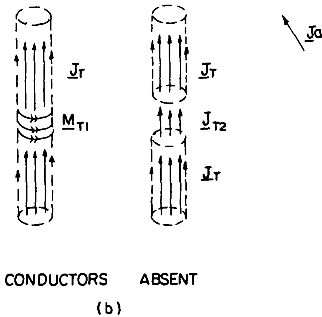
Fig. 3-6. The two-port receiving antenna with mixed sources (a) conductors present (b) conductors absent.
