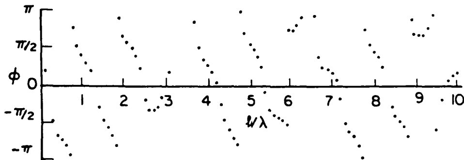
Fig. 2-22. Current distribution for a VEE scatterer ( \theta_0 = 90^\circ , \phi_0 = 270^\circ )
