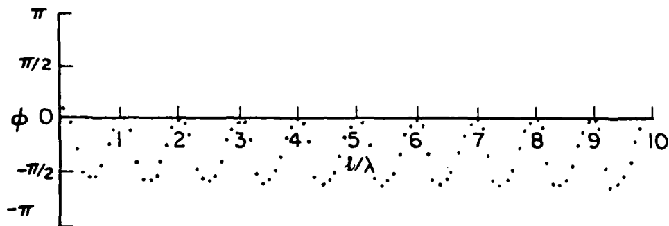
Fig. 2-19. Current distribution for a VEE scatterer ( \theta_0 = 45^\circ , \phi = 90^\circ )
