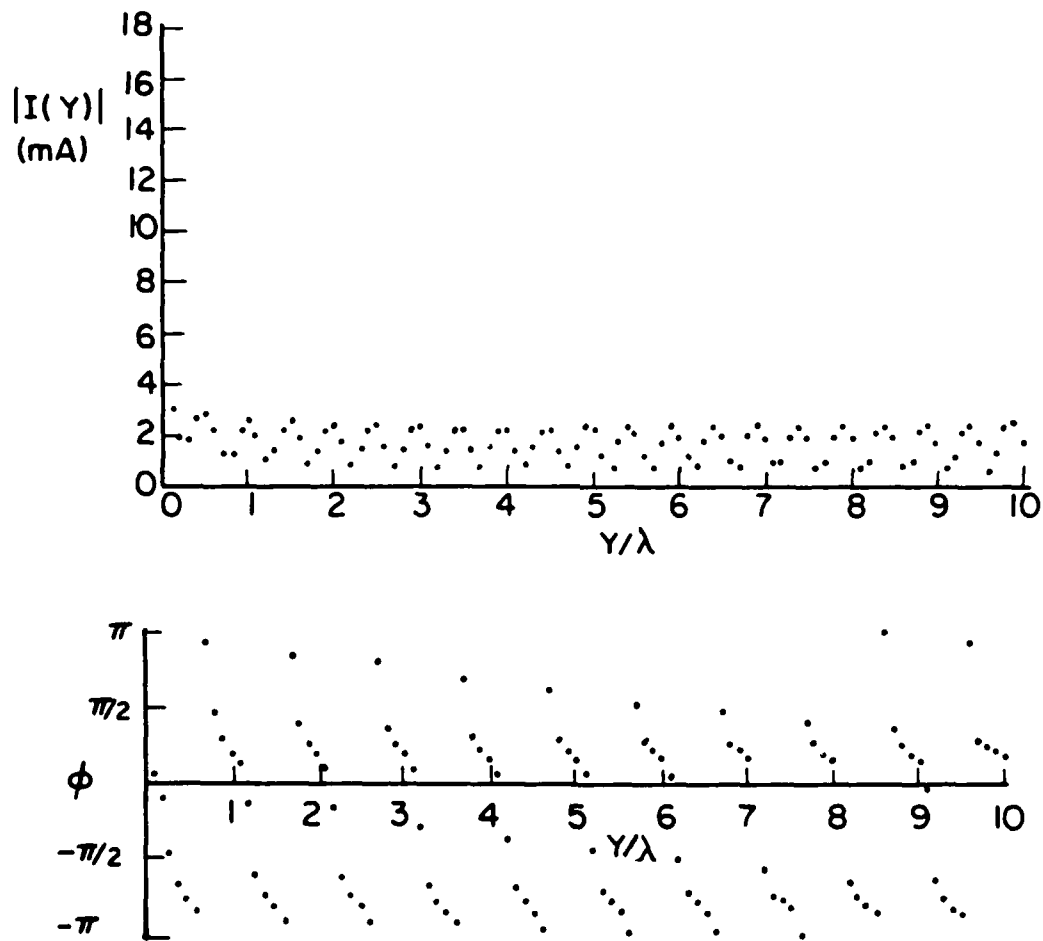
Fig. 2-13. Current distribution for a transmission line radiator ( 2d = 2.0\lambda , Z_t = \infty ).
