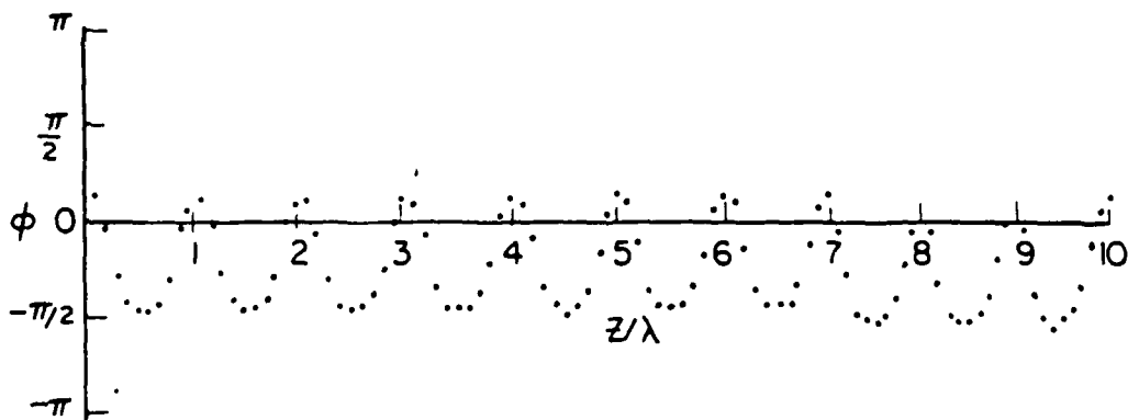
Fig. 2-24. Current distribution for a dipole scatterer ( \theta_0 = 90^\circ , \phi_0 = 270^\circ )
