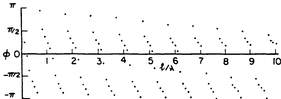
Fig.2-17. Current distribution for a VEE radiator.
