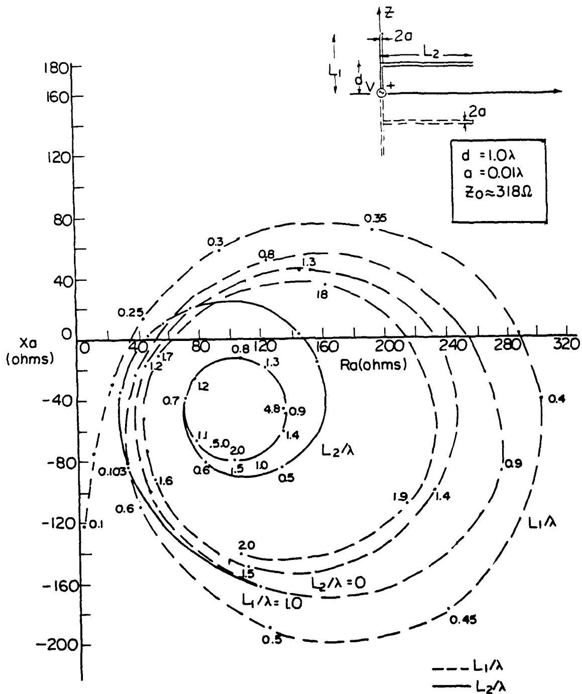
Fig. 4-3. Impedance of the dipole/transmission line ( d = 1.0\lambda ).
