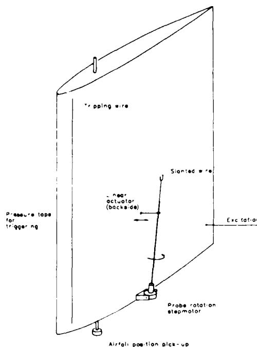
Figure 1. Experimental set-up.
